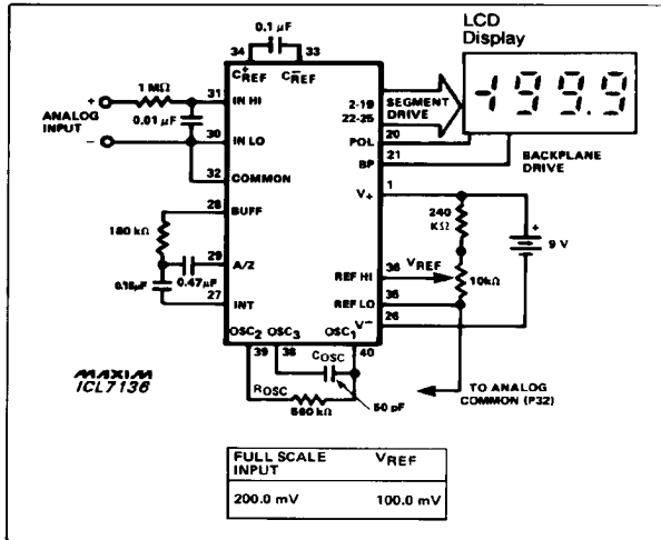
Figure 1. Maxm ICL7136 Typical Operating Circuit Clock Frequency 16kHz (1 reading/sec)
