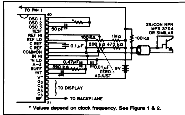
Figure 11. 7136 used as a Digital Centigrade Thermometer. A silicon diode-connected transistor has a temperature coefficient of about -2\text{mV}/^\circ\text{C} . Calibration is achieved by placing the sensing transistor in ice water and adjusting the zeroing potentiometer for a 000.0 reading. The sensor should then be placed in boiling water and the scale-factor potentiometer adjusted for a 100.0 reading.
