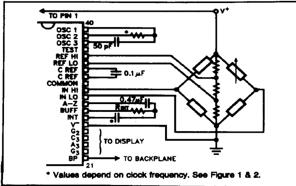
Figure 10. 7136 Measuring Ratiometric Values of Quad Load Cell. The resistor values within the bridge are determined by the desired sensitivity.
