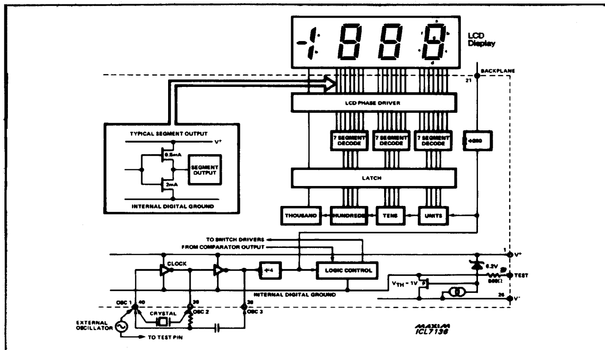
Figure 7. ICL7136 Digital Section
