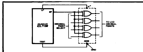
Figure 6. Exclusive "OR" Gate for Decimal Point Drive
