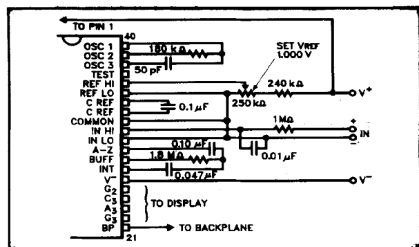
Figure 8. Recommended Component Values for 2.000V Full-Scale, 3 Readings/Sec. For 1 reading/sec, change CINT, ROSC to values of Figure 1.
