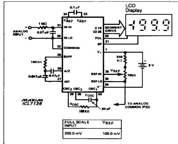
Figure 2. Maxm ICL7136 Typical Operating Circuit Clock Frequency 48kHz (3 readings/sec)
