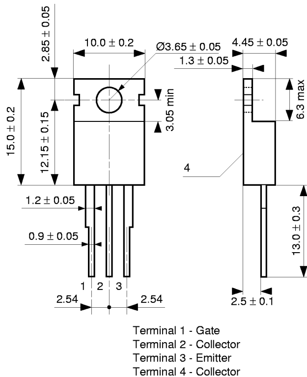
Package OutlineType: TO220
