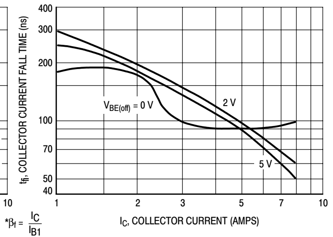
Figure 14. Collector Current Fall Time
