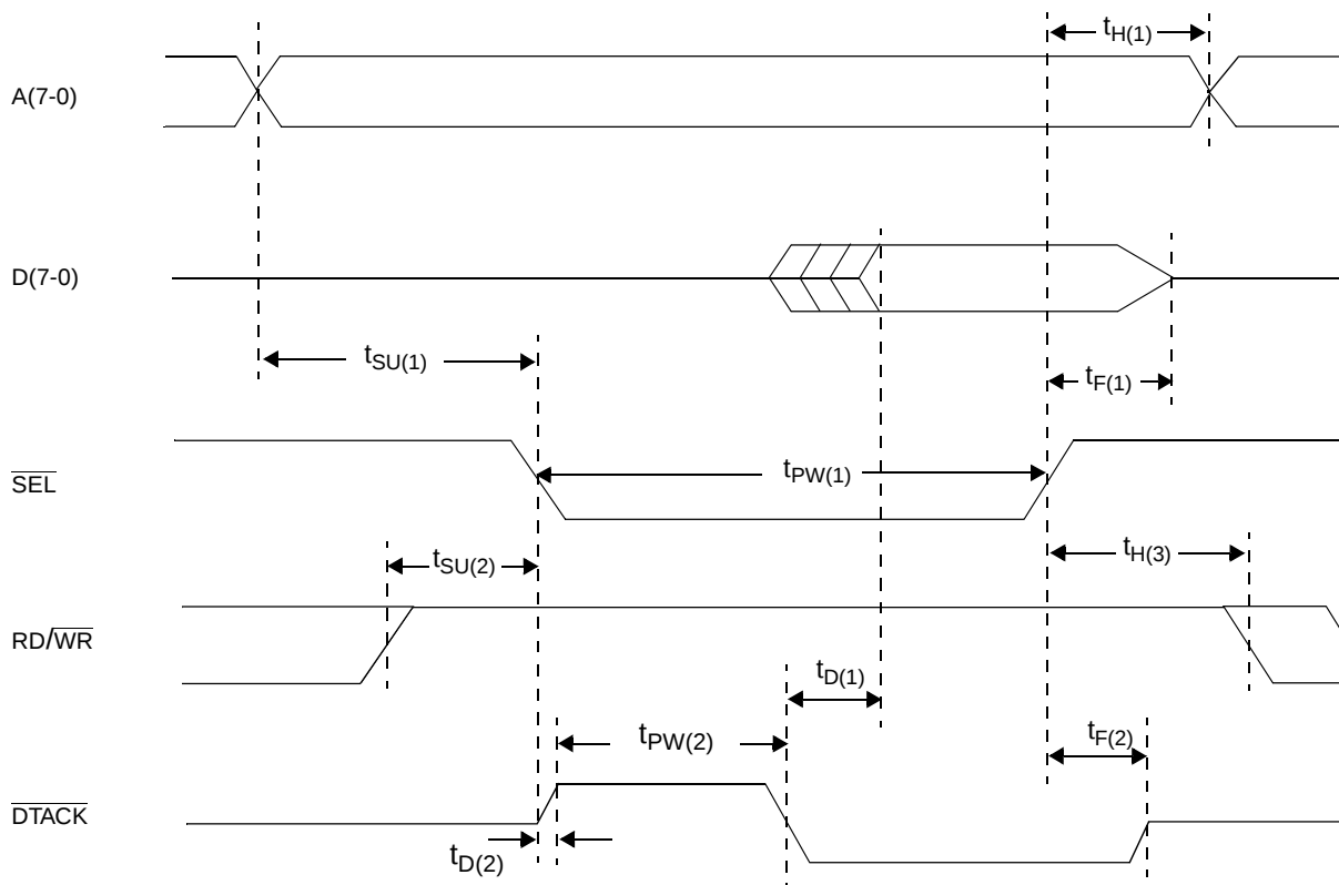
Figure 27. Motorola Microprocessor Read Cycle Timing
