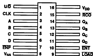
16-Lead Flatpack Top View
