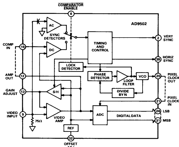
AD9502 FUNCTIONAL BLOCK DIAGRAM
