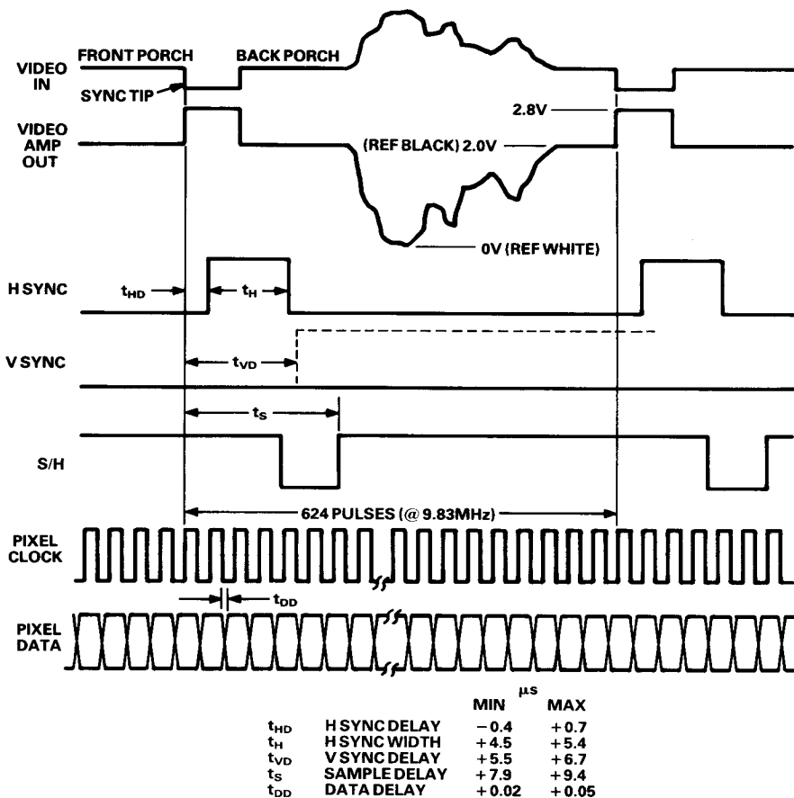
Figure 1. AD9502 Timing Diagram
