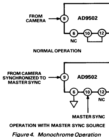
Figure 4. Monochrome Operation
