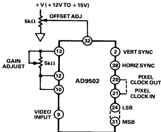
Figure 2. Offset and Gain Adjustments
