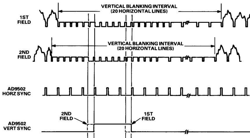
Figure 3. Field/Sync Timing Diagram
