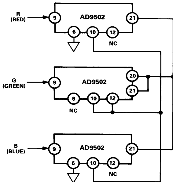
Figure 5. RGB Operation (External Pixel Clock)
