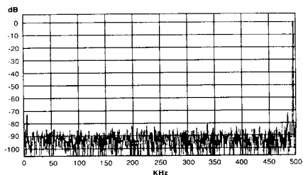
FFT Analysis of ADS-193
