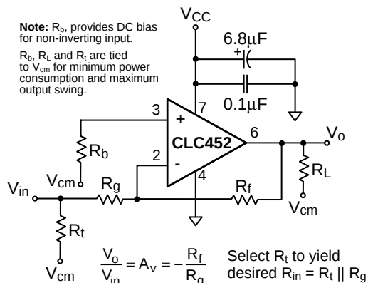
Figure 2: Inverting Configuration
