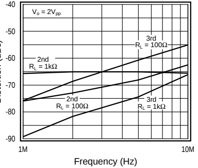
2nd Harmonic Distortion, R_L = 100\Omega
