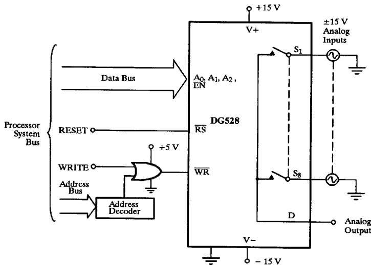
Figure 9. Bus Interface
