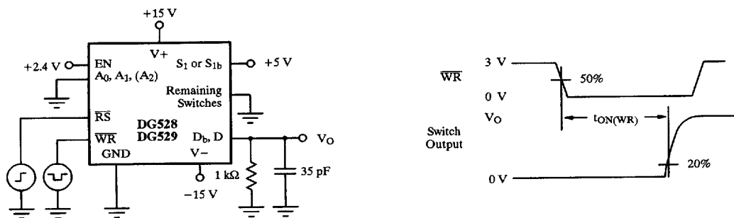
Figure 7. Write Turn-On Time t_{ON(WR)}
