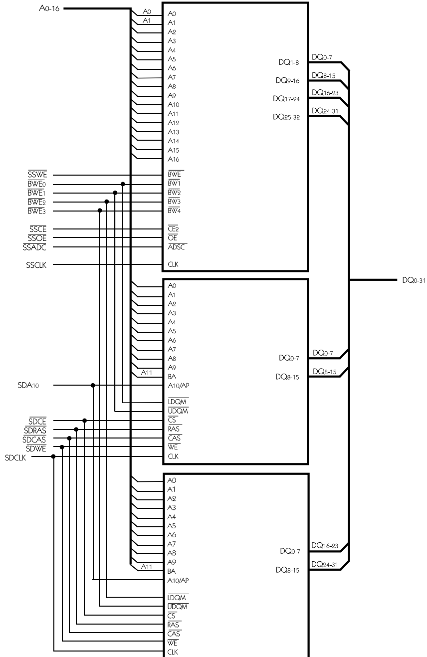
FIG. 2 BLOCK DIAGRAM
