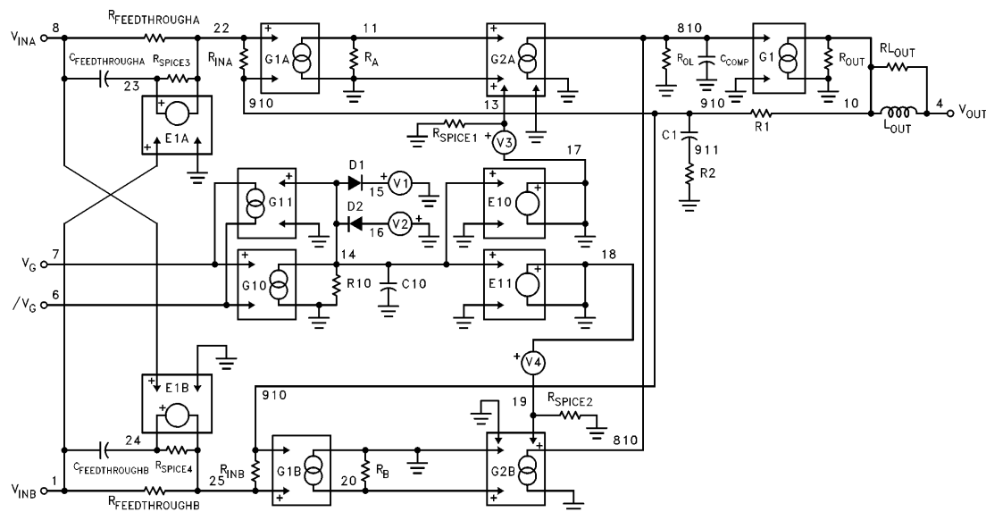
EL4094 Macromodel Schematic
