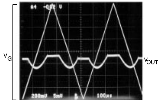
Cross-Fade Balance. V_{\text{INA}} = V_{\text{INB}} = 0 \text{ V}
