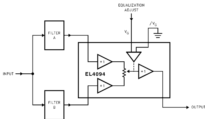
General Adjustable Equalizer
