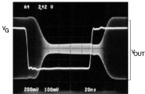
Gain Control Response to a Non-Overloading Step, Constant Sinewave at V_{\text{INA}}
