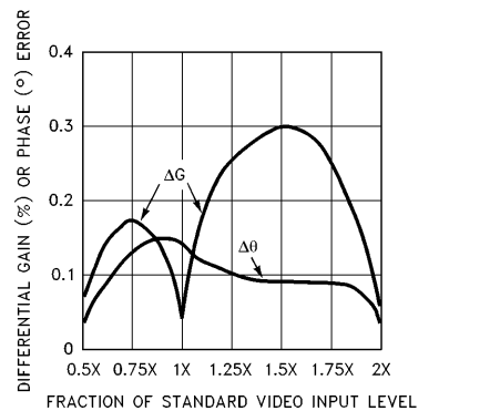
Differential Gain and Phase of Linearized Level Control
