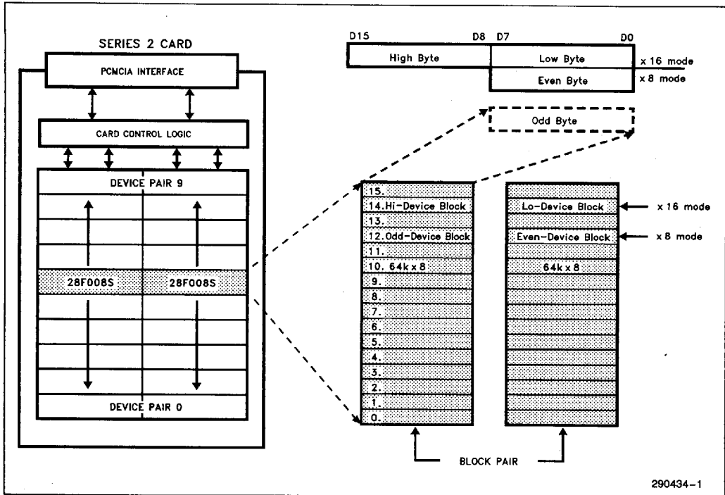
Figure 2. Memory Architecture. Each Device Pair Consists of Sixteen 64 KWord Blocks.
