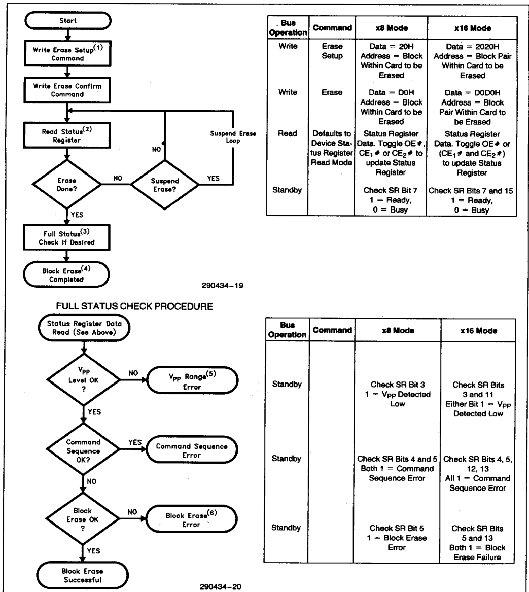
Figure 14. Device-Level Automated Erase Algorithm
