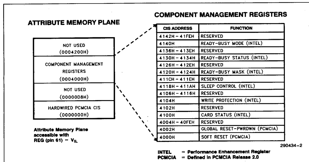
Figure 3. Component Management Registers Allow S/W Control of Components within Card
