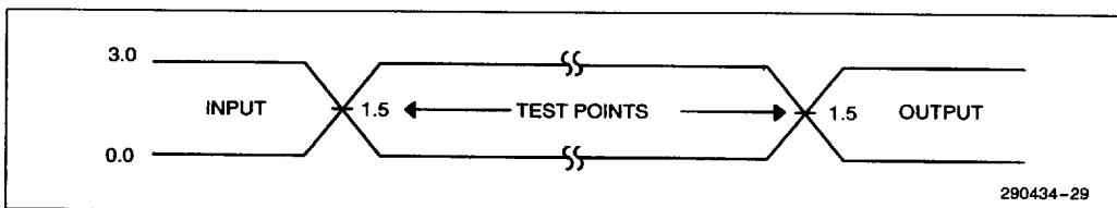
Transient Input/Output Reference Waveform ( V_{CC} = 3.3V ) for Standard Test Configuration
