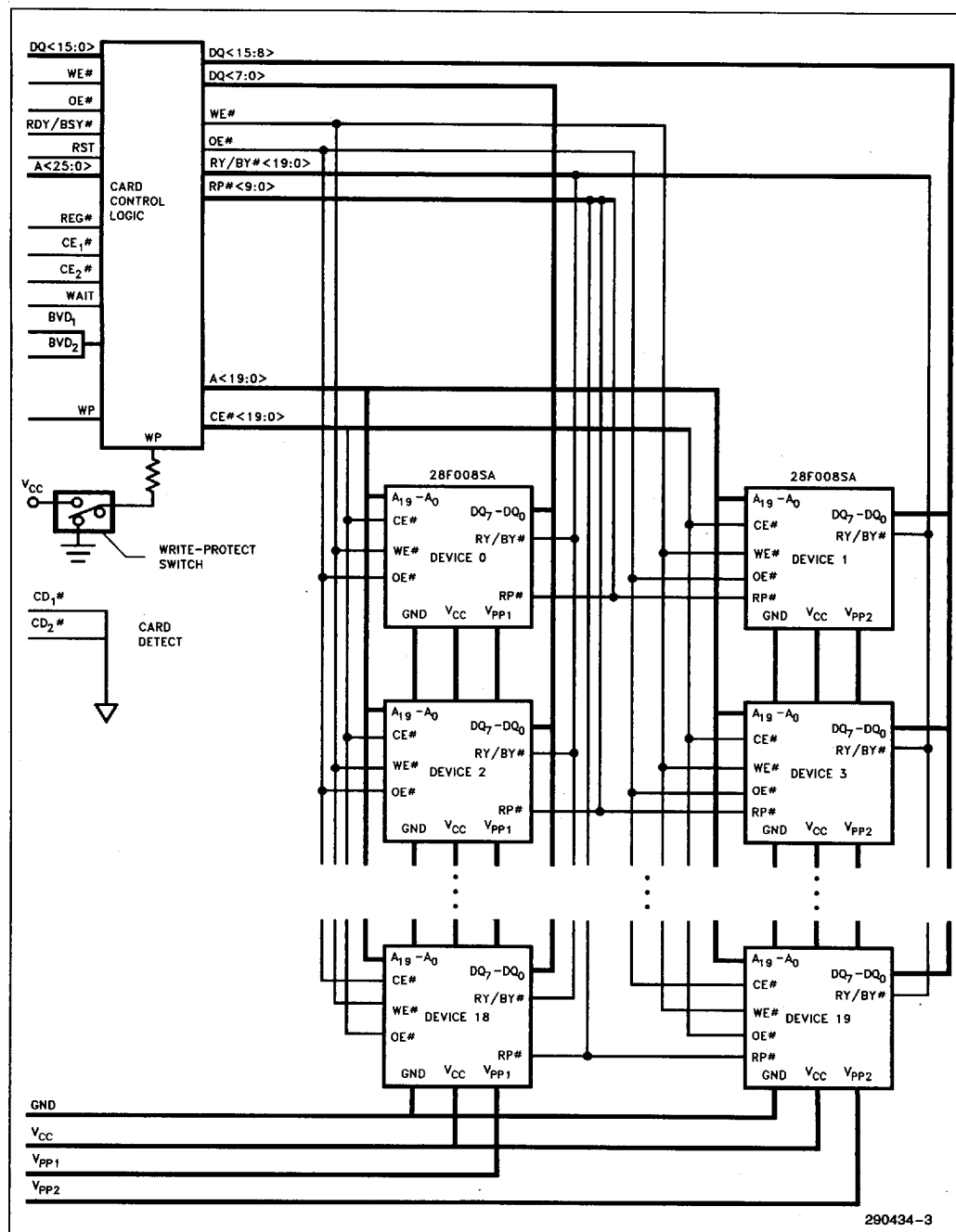
Figure 1. Detailed Block Diagram. The Card Control Logic Provides Decoding Buffering and Control Signals.
