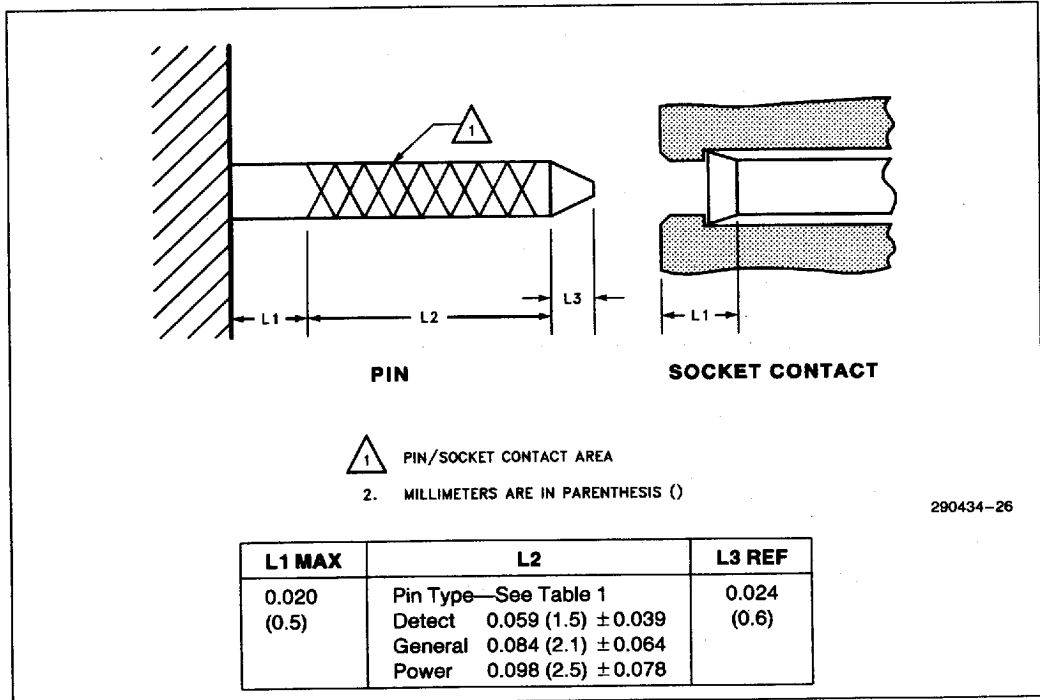
Figure 21. Pin/Socket Contact Length with Wipe
