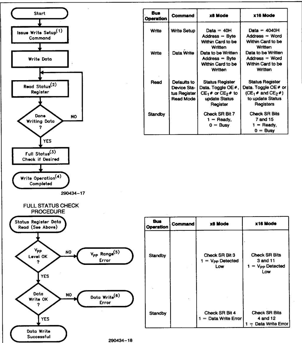
Figure 13. Device-Level Automated Write Algorithm
