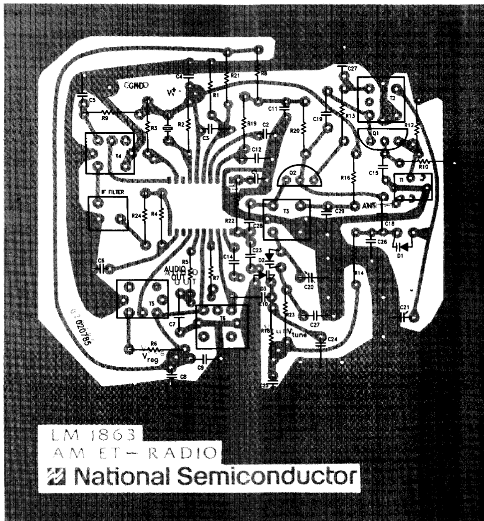
PC Layout (Component Side)
