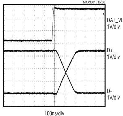
DRIVER PROPAGATION DELAY LOW-TO-HIGH (LOW-SPEED MODE)
