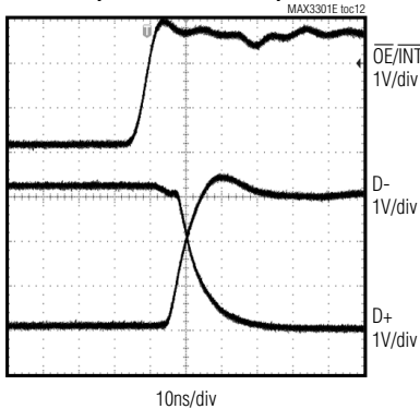
DRIVER DISABLE DELAY (FULL-SPEED MODE)
