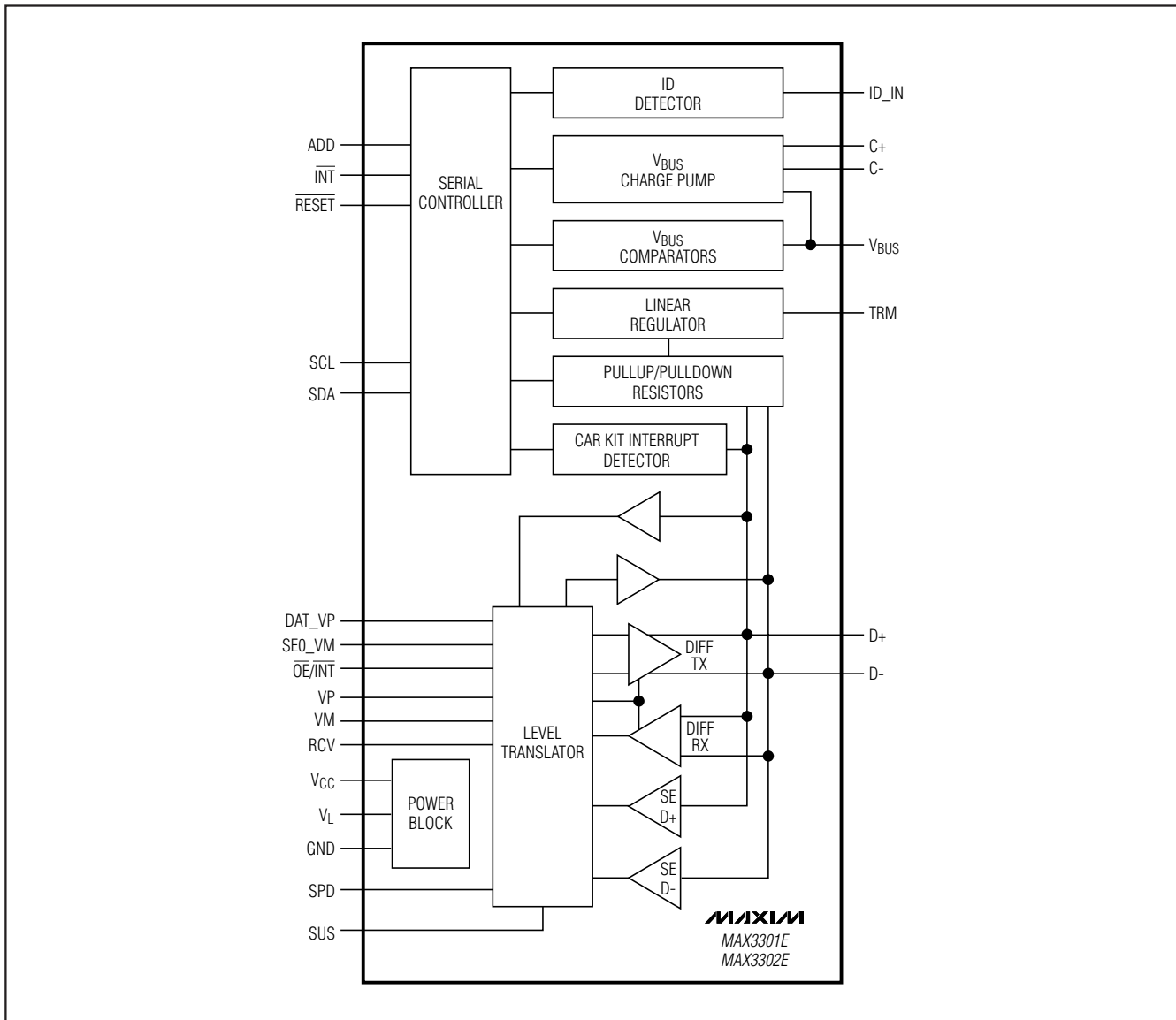
Figure 11. Block Diagram
