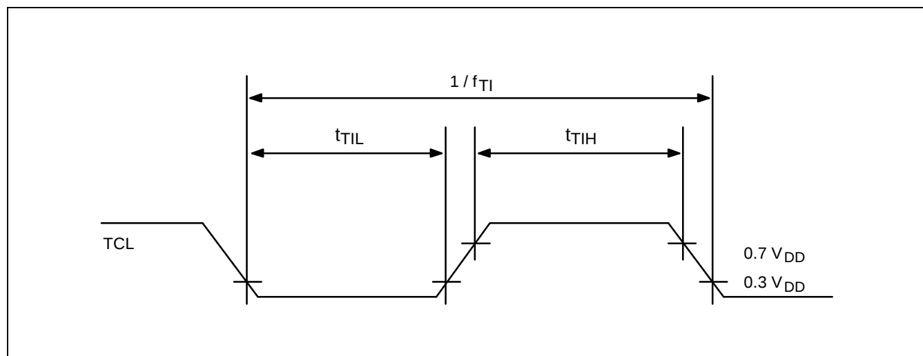
Figure 14-6. TCL Timing
