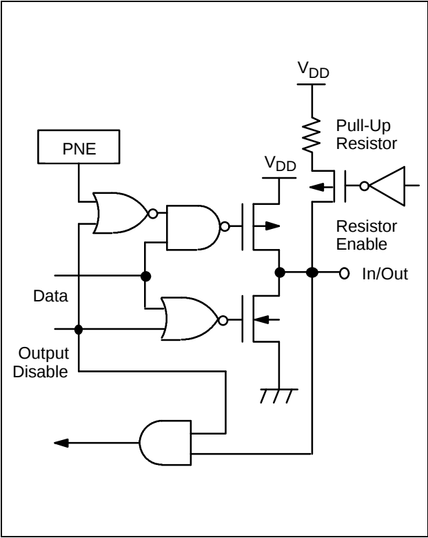
Figure 1-8. Pin Circuit Type E-2
