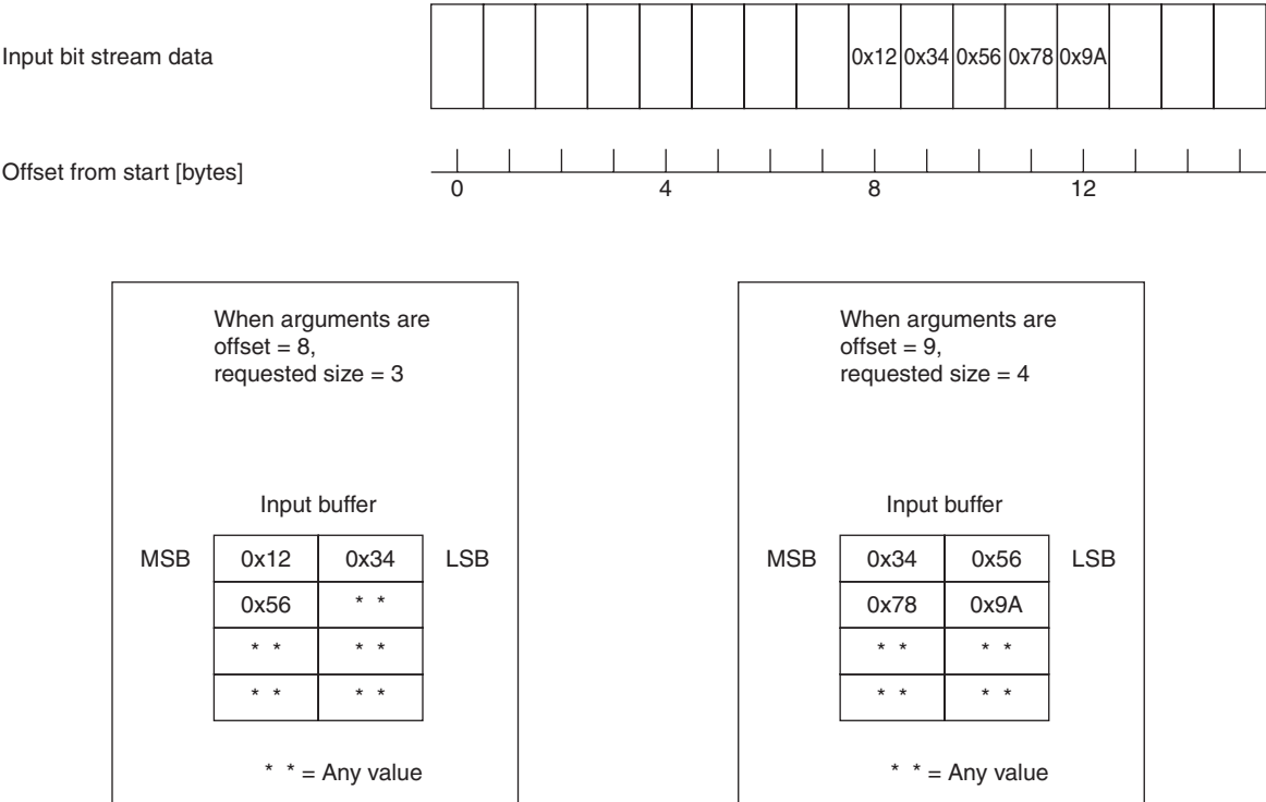
Figure 2-2. Setting Data in Input Buffer
