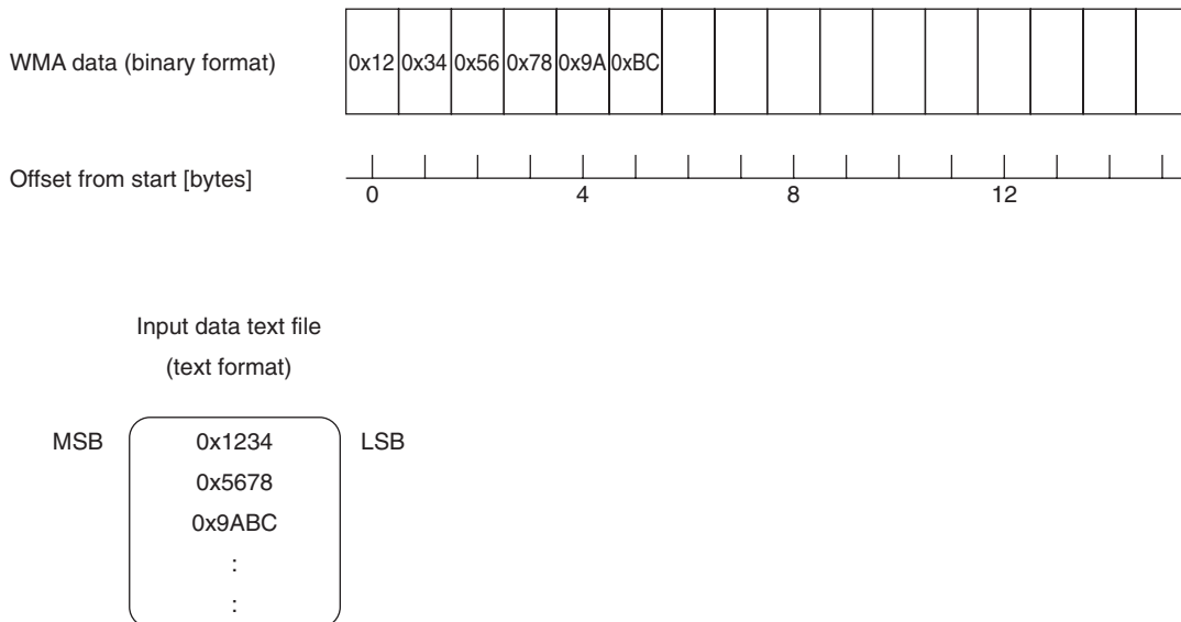
Figure 4-1. Input Data File
