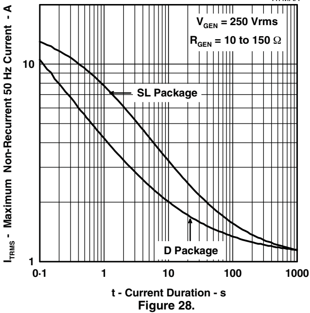
TISP7125F3 THRU TISP7180F3 MAXIMUM NON-RECURRING 50 Hz CURRENT vs CURRENT DURATION
