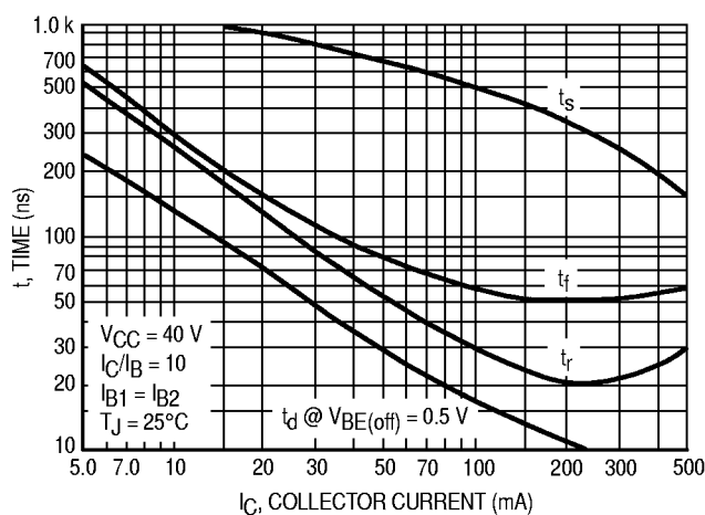
Figure 4. Switching Time
