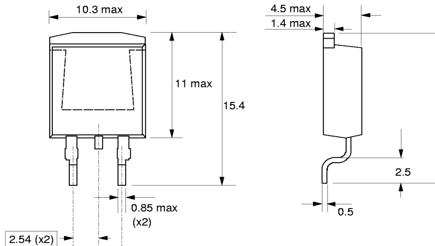
Fig.13. SOT404 : centre pin connected to mounting base.
