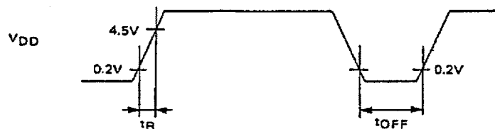
Fig. 8 Power on reset
