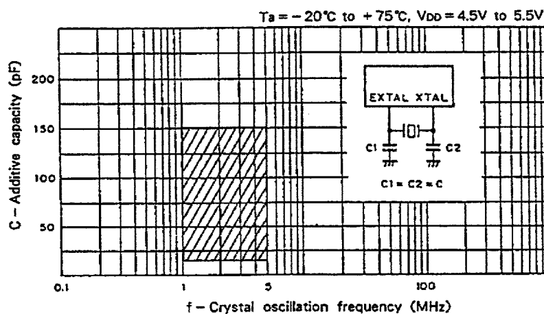
Fig. 9 Crystal oscillator circuit additive capacity calculation chart
