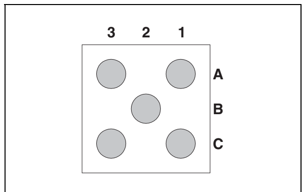
Figure 2: Pin Configuration (Bump Side)
