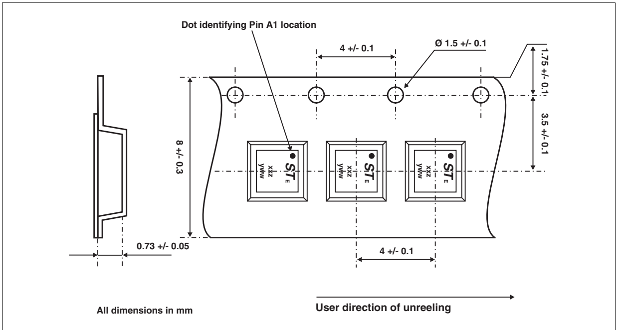
Figure 16: FLIP-CHIP Tape and Reel Specification
