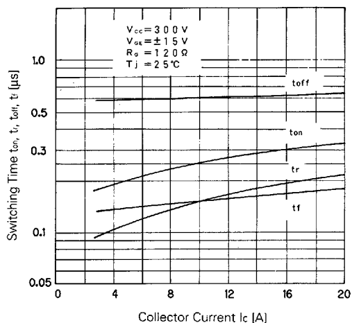
Switching Time
