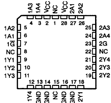
54AC11241 . . . FK PACKAGE (TOP VIEW)
