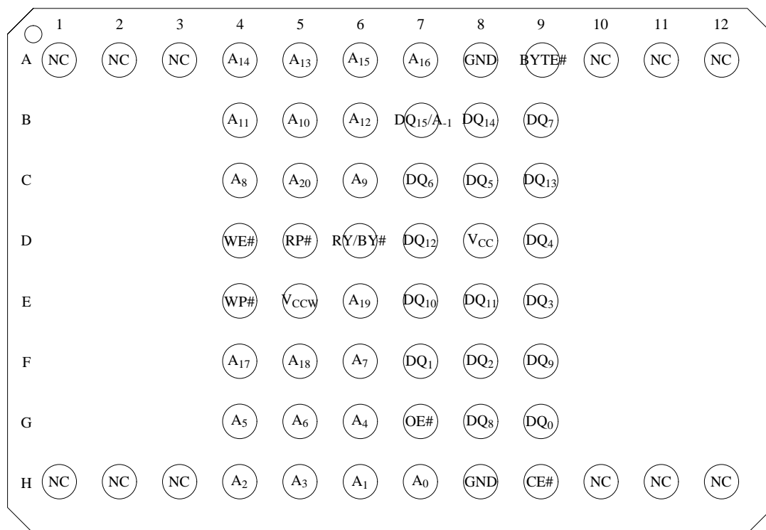
Figure 2. CSP 60-Ball Pinout
