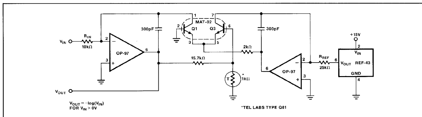
FIGURE 12: Low Power Logarithmic Amplifier
