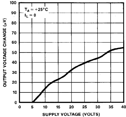
OUTPUT VOLTAGE CHANGE vs SUPPLY VOLTAGE
