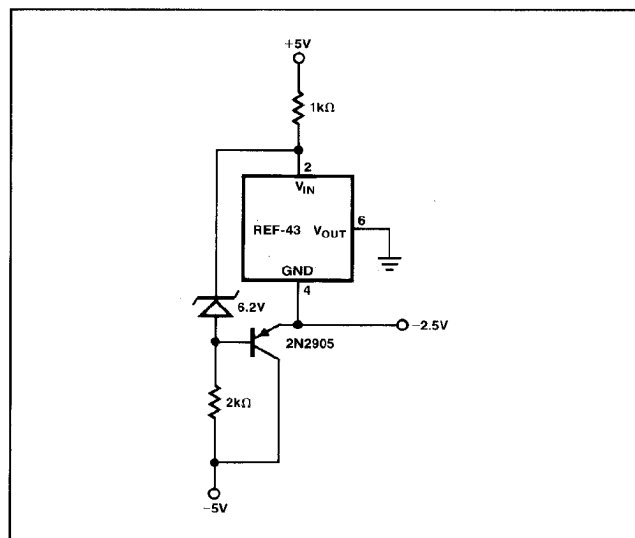
FIGURE 4: -2.5V Reference
