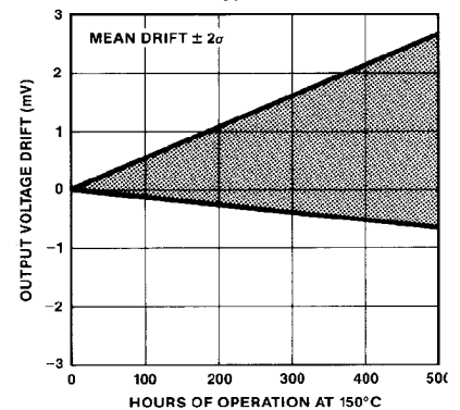
BURN-IN DRIFT AT T_A = 150^{\circ}\text{C}
