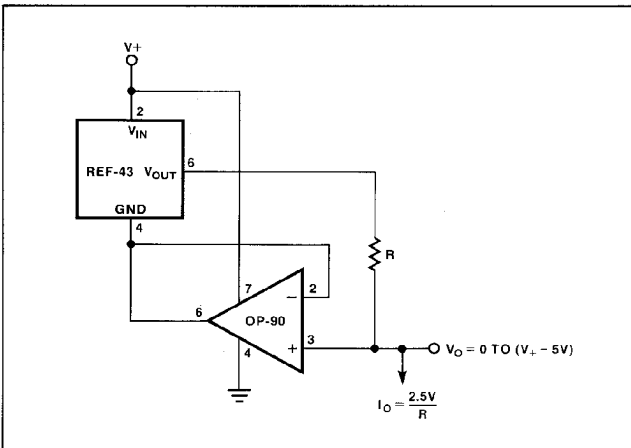
FIGURE 7: Precision Current Source
