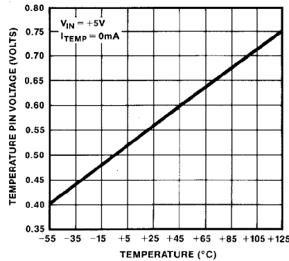
TEMPERATURE PIN VOLTAGE vs TEMPERATURE
