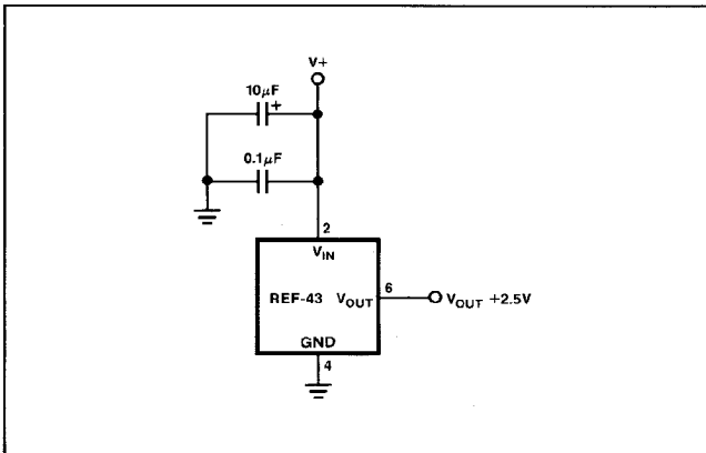
FIGURE 1: Basic Connections
