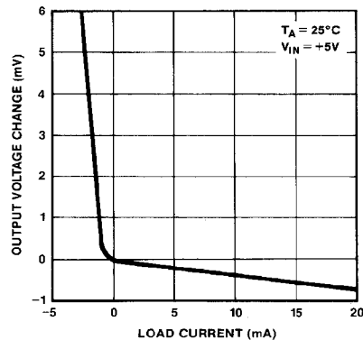
OUTPUT VOLTAGE CHANGE vs LOAD CURRENT
