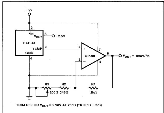
FIGURE 8: Single-Supply Kelvin-Output Thermometer
