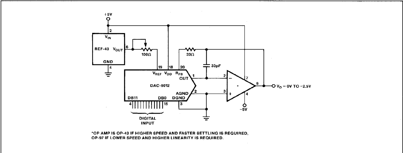
FIGURE 6: CMOS DAC Reference
