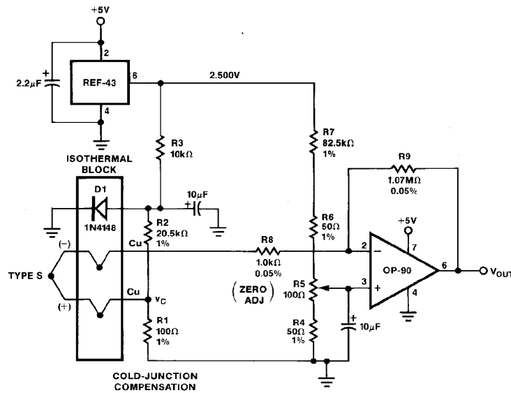
FIGURE 9: Thermocouple Amplifier with Cold-Junction Compensation
