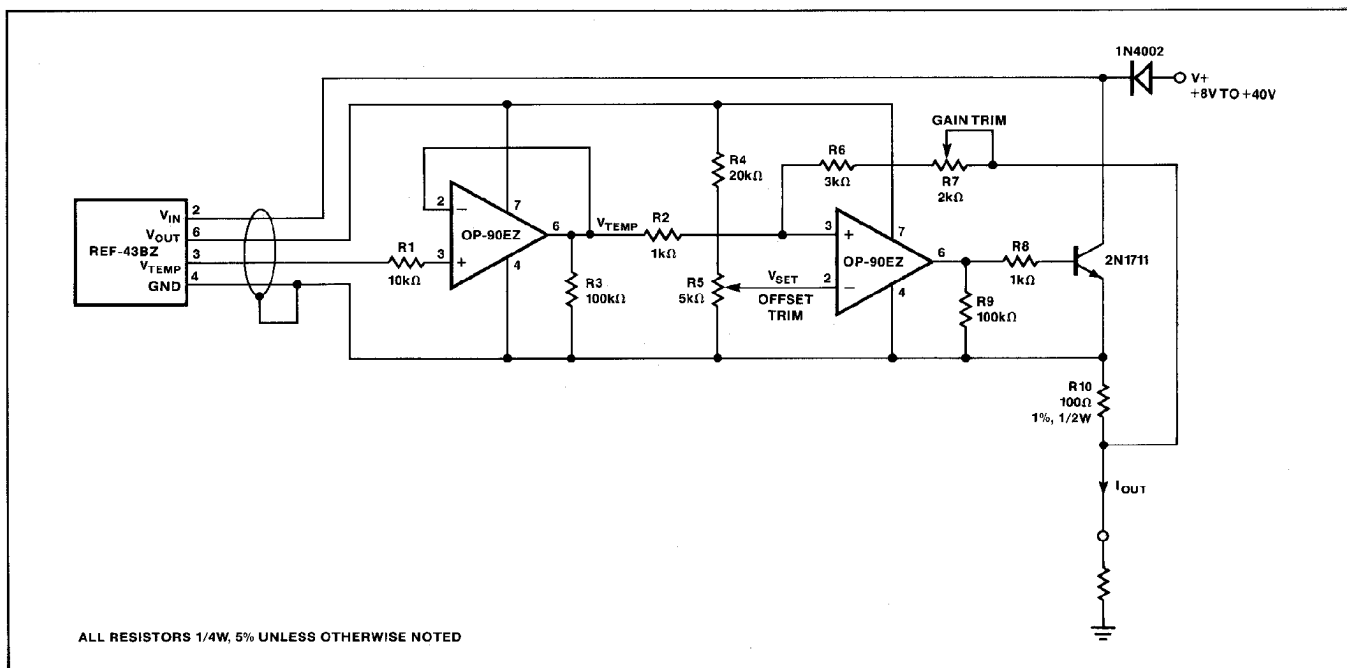
FIGURE 11: Temperature to 4-20mA Transmitter
