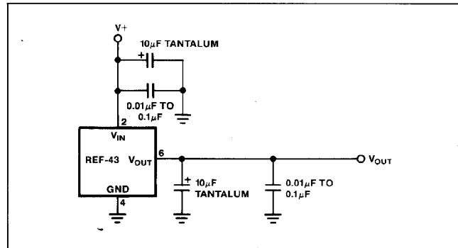
FIGURE 2A: Recommended Decoupling for High-Frequency Pulse Response
