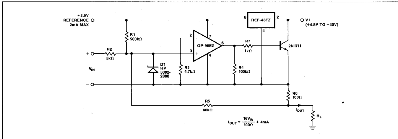
FIGURE 10: Two Wire 4-20mA Transmitter
