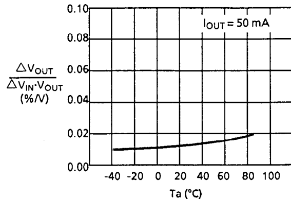
2.12 Input stability ( V_{OUT} ) - Temperature
