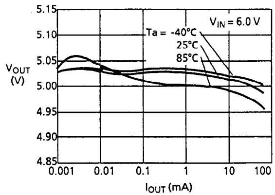
2.6 Output current ( I_{OUT} ) - Output voltage ( V_{OUT} )
