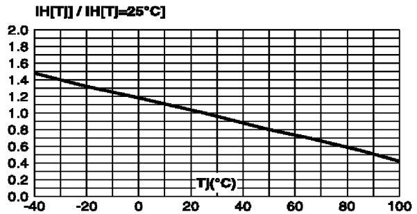
Fig. 2: Relative variation of holding current versus junction temperature.
