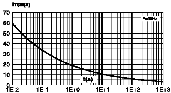
Fig. 1: Non repetitive surge peak on-state current versus overload duration ( T_j initial=25°C).
