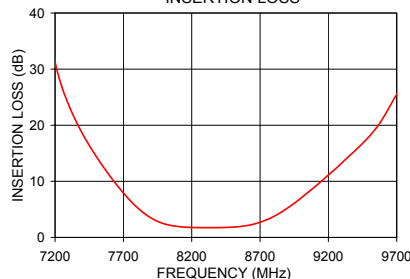
VBF-8350+ INSERTION LOSS
