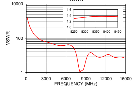
VBF-8350+ VSWR
