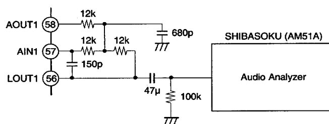
LPF external circuit diagram
