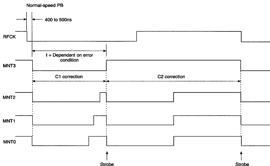
Timing Chart 4-3
