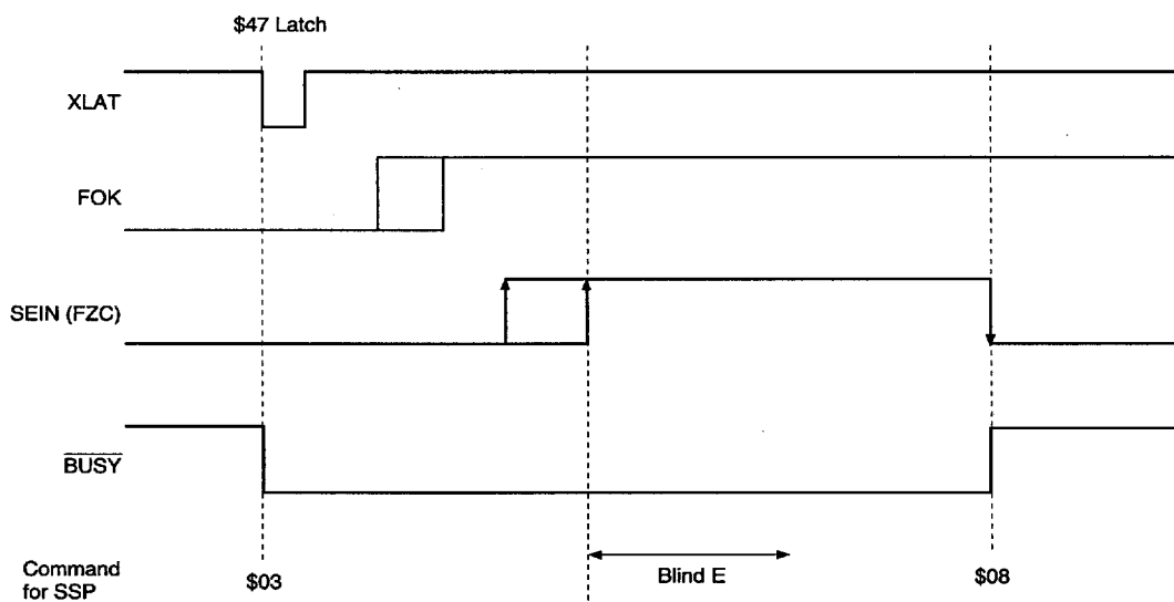
Fig. 4-8 (b). Auto Focus Timing Chart
