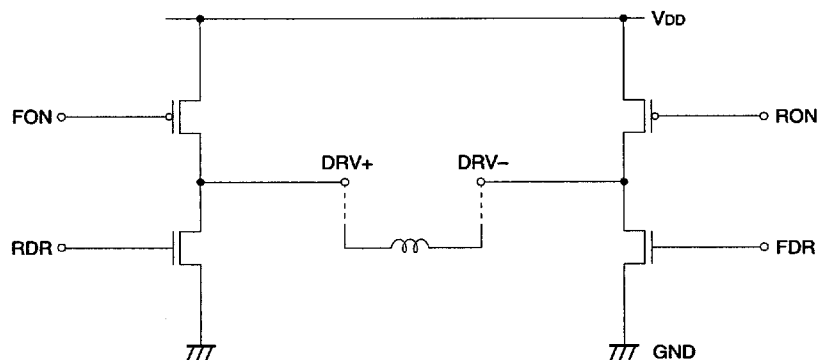
Fig. 5-21. PWM Bridge Drive Circuit
