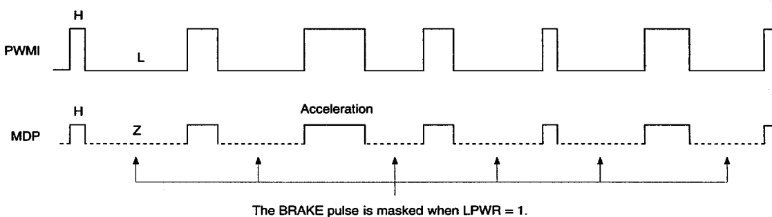
Timing Chart 1-20
