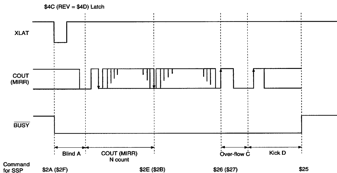
Fig. 4-11 (b). 2N Track Jump Timing Chart
