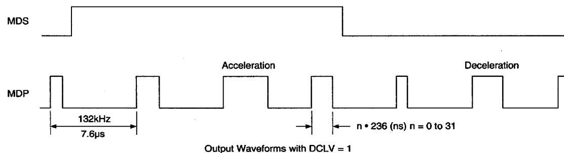
Timing Chart 1-14
