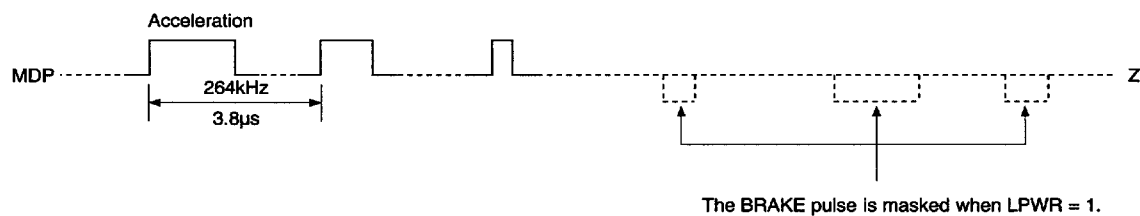
Timing Chart 1-18
