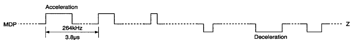
Timing Chart 1-18
