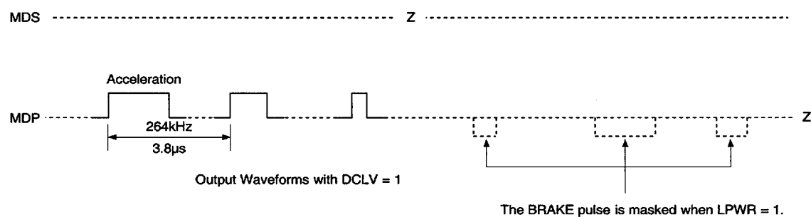
Timing Chart 1-17
