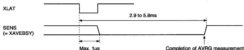
Timing Chart 5-2.
