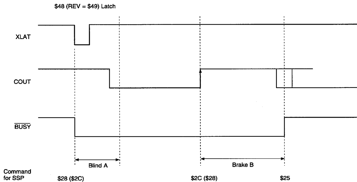
Fig. 4-9 (b). 1-Track Jump Timing Chart
