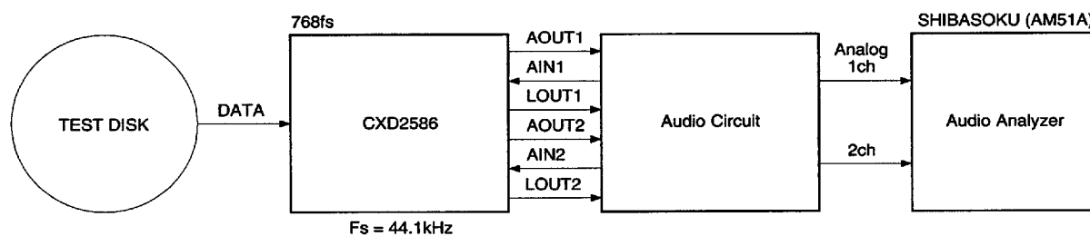
Block diagram of analog characteristics measurement
