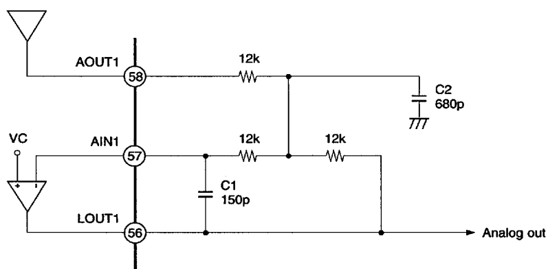
LPF external circuit
