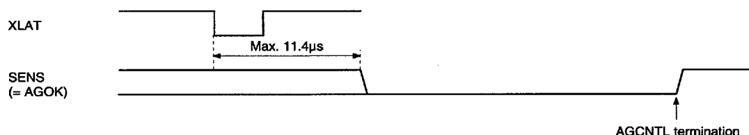
Timing Chart 5-4.
