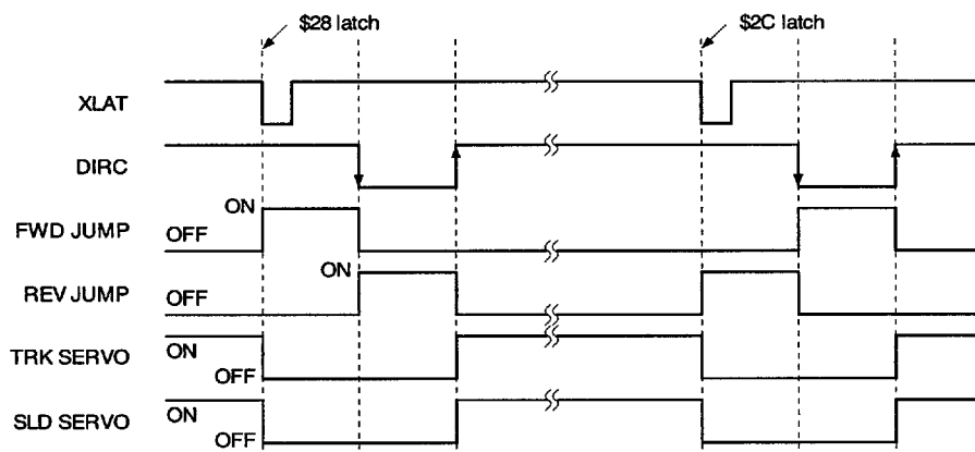
Timing Chart 5-24.
