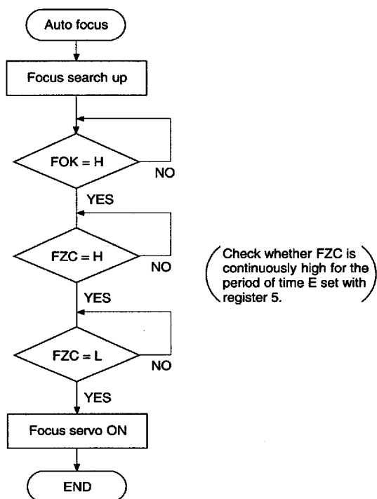
Fig. 4-8 (a). Auto Focus Flow Chart
