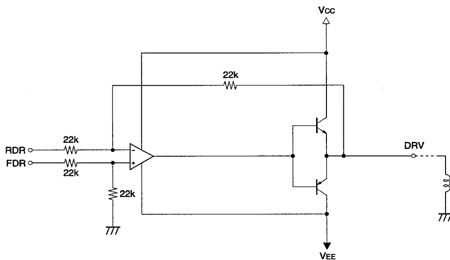
Fig. 5-22. Operational Amplifier Drive Circuit
