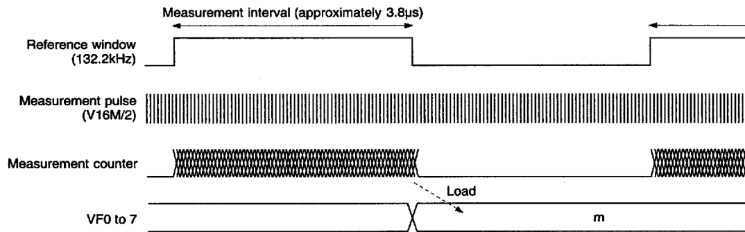
Timing Chart 2-5
