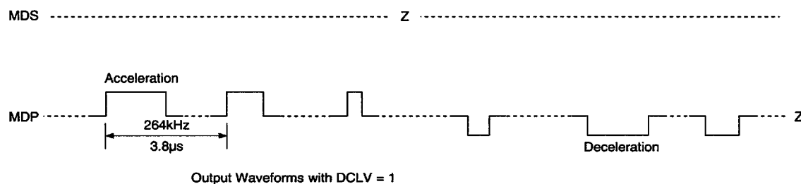
Timing Chart 1-16
