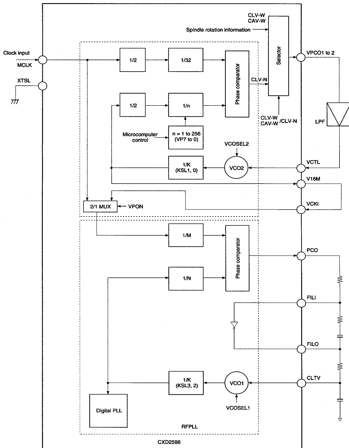
Block Diagram 4-1
