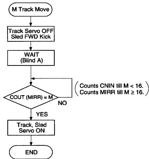
Fig. 4-13 (a). M-Track Move Flow Chart
