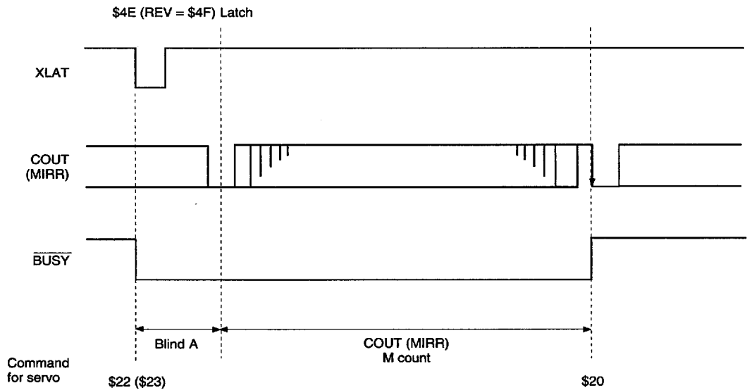
Fig. 4-13 (b). M-Track Move Timing Chart
