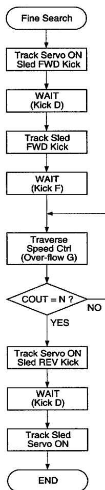
Fig. 4-12 (a). Fine Search Flow Chart
