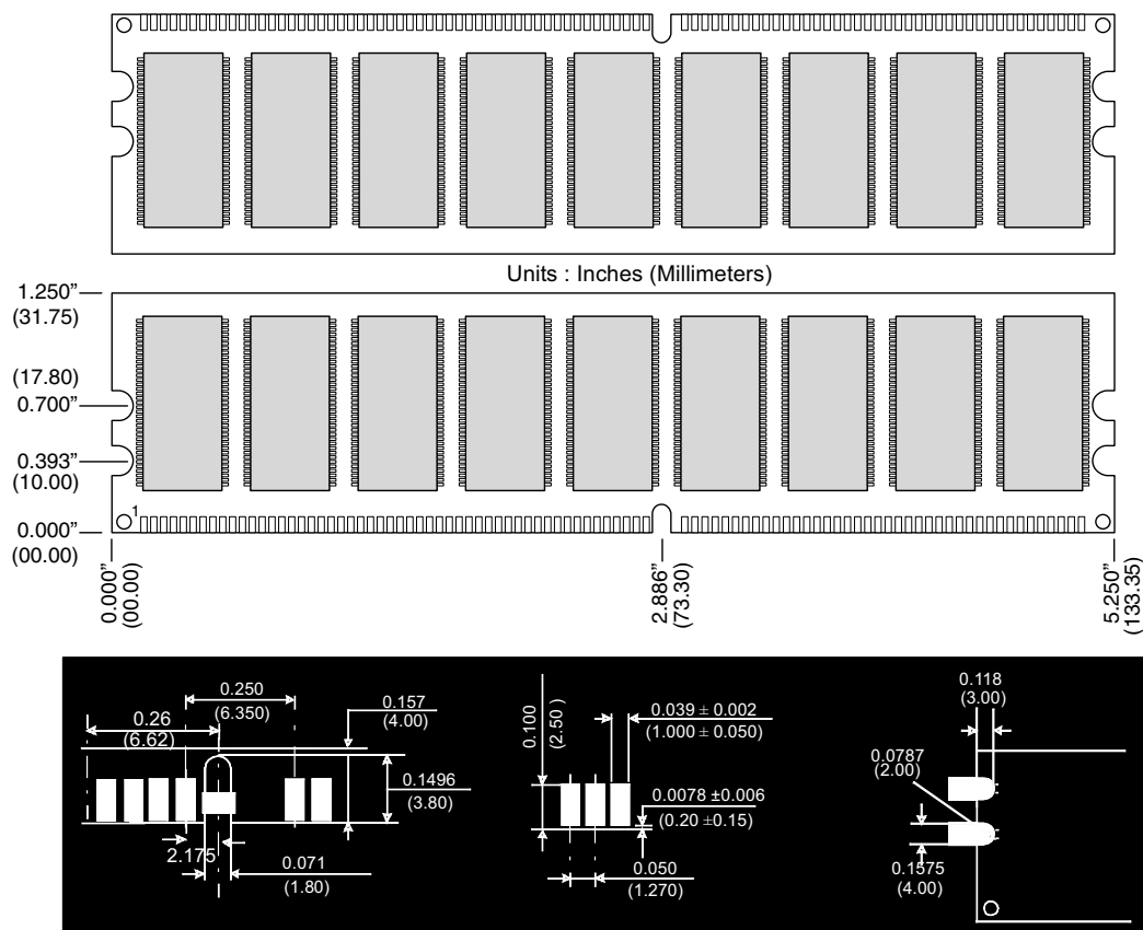
Figure 1: KVR266X72C25/512 184-Pin DDR SDRAM Module
