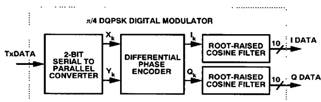
Figure 9. \pi/4 DQPSK Modulator Functional Block Diagram
