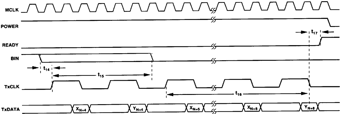
Figure 5. Transmit Timing at the End of a Tx Burst
