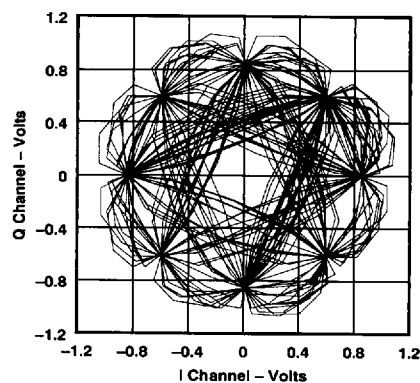
Figure 17. AD7011 I vs. Q Waveforms Filtered by an Ideal Root Raised Cosine Receive Filter
