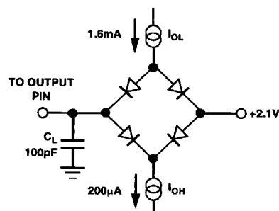
Figure 3. Load Circuit for Digital Outputs
