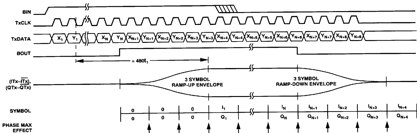
Figure 12. Transmit Burst
