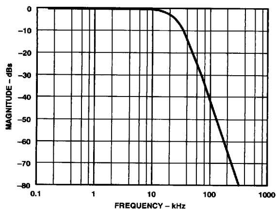
Figure 13. Reconstruction Filter Frequency Response for the I and Q DACs, MCLK = 2.56 MHz
