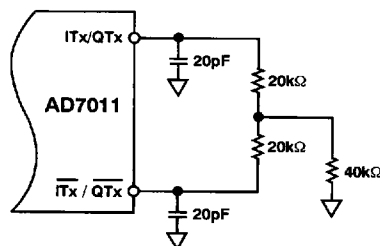
Figure 1. Analog Output Test Load Circuit
