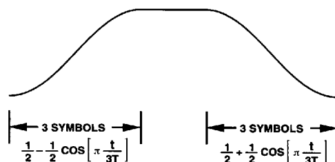
Figure 11. Ramp Envelope
