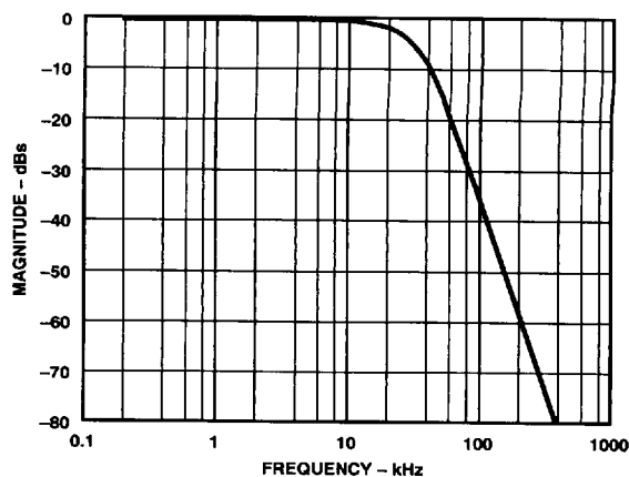
Figure 16. Reconstruction Filter Frequency Response for the I and Q DACs, MCLK = 3.1104 MHz
