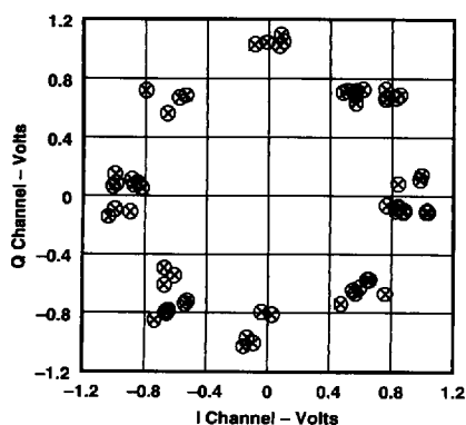
Figure 15. AD7011 Transmit Constellation Diagram
