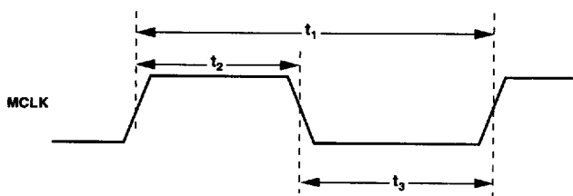
Figure 2. Master Clock (MCLK) Timing
