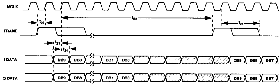
Figure 6. Analog Mode Serial Interface Timing
