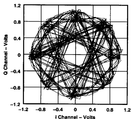
Figure 14. AD7011 I vs. Q Waveforms When Transmitting Random Data
