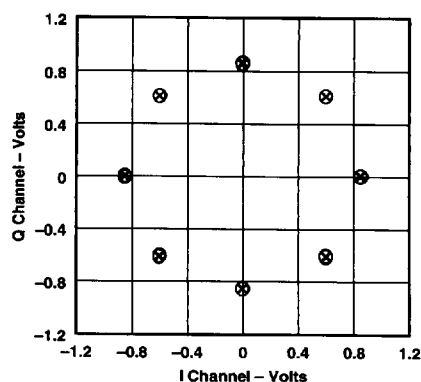
Figure 18. AD7011 Constellation Diagram When Filtered by an Ideal Root Raised Cosine Receive Filter
