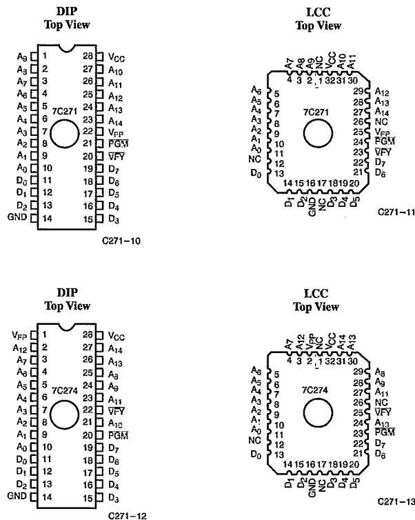
Figure 1. Programming Pinouts
