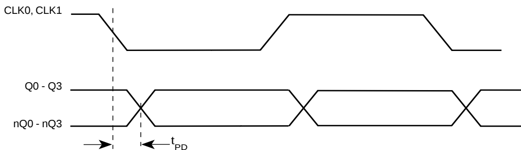
FIGURE 6 - PROPAGATION DELAY
