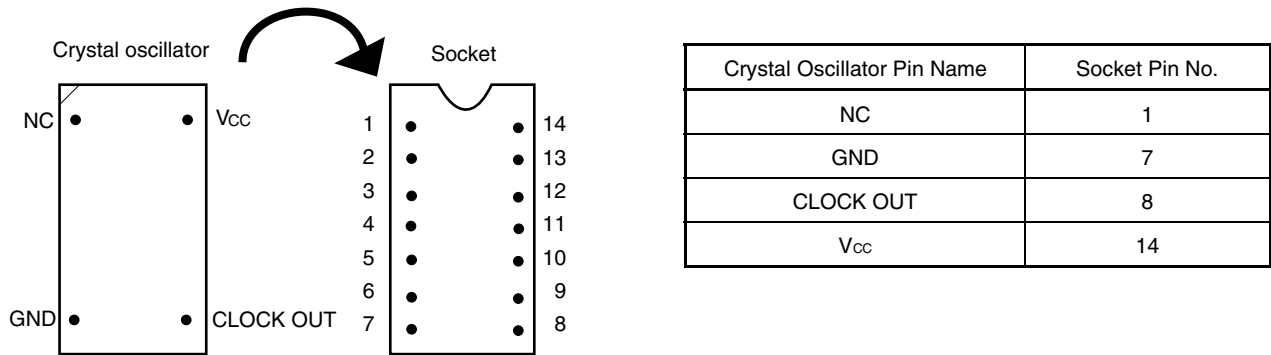
Figure 3-11. Pin Alignment of Crystal Oscillator and Socket (Main System Clock)
