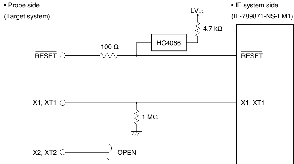
Figure 4-2. Equivalent Circuit 2 of Emulation Circuit
