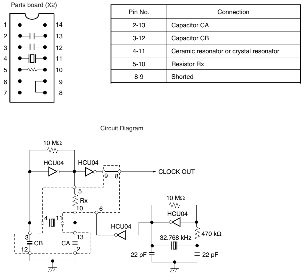
Figure 3-12. Connections on Parts Board (Subsystem Clock)
