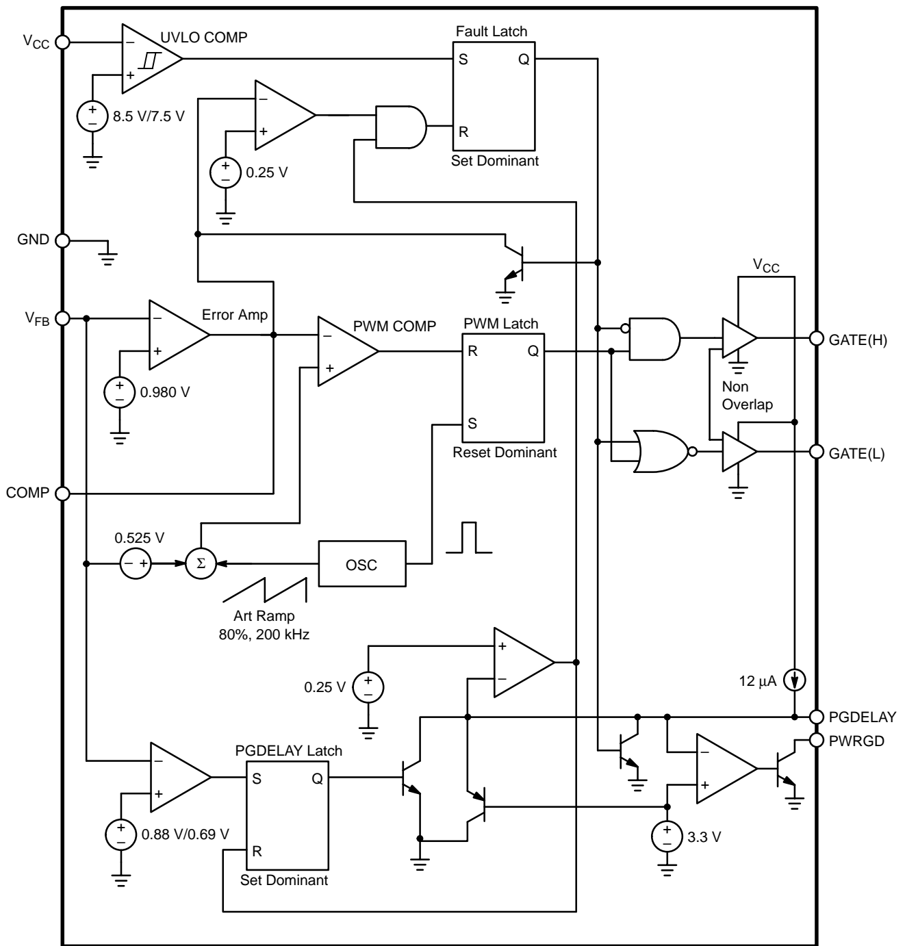
Figure 2. Block Diagram
