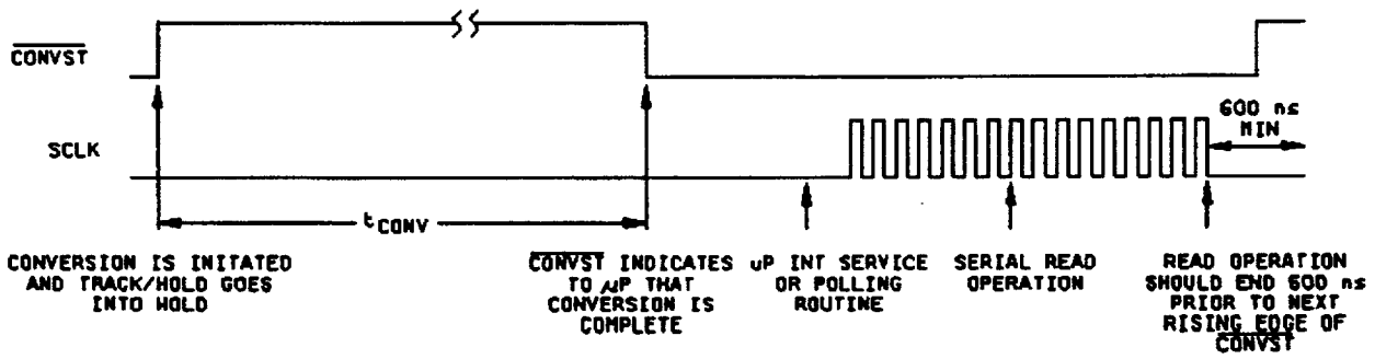
CONVST USED AS STATUS SIGNAL
