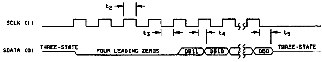
DATA READ OPERATION
