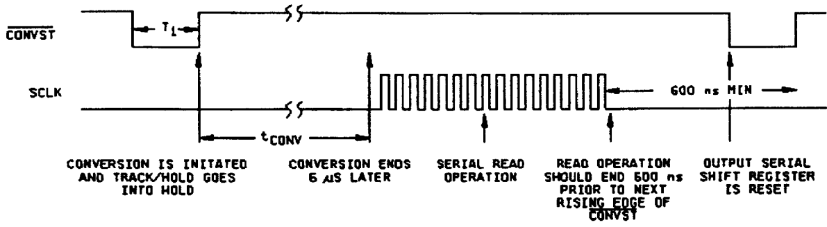
TIMING SEQUENCE FOR OPTIMUM PERFORMANCE
