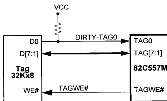
Figure 4-18 32Kx8 Combined Tag/Dirty RAM Implementation
