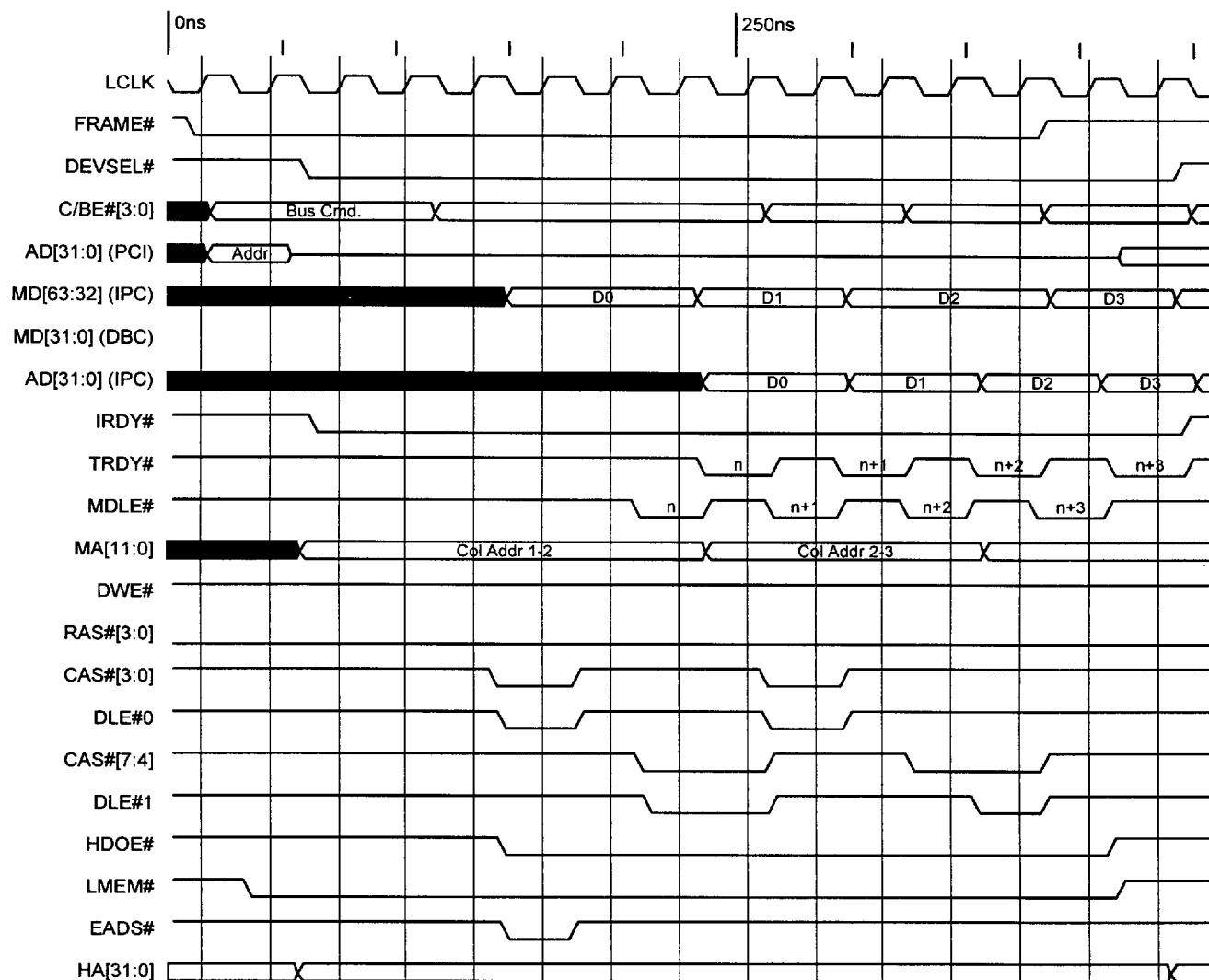
Figure 4-26 PCI Master Read from Local Memory
