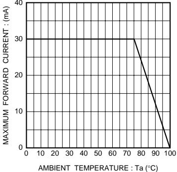
Fig.7 Derating
