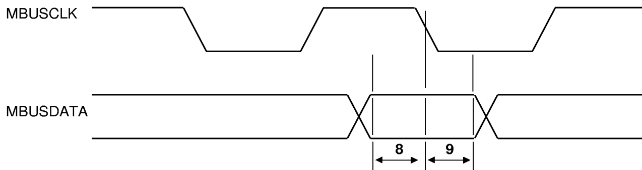
Magic Bus Input Timing (Slave, RCVPHAPOL=1)
