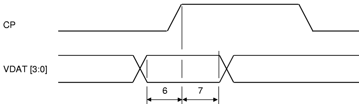
Video Data Timing, 4 bit split LCD and 8 bit non-split LCD
