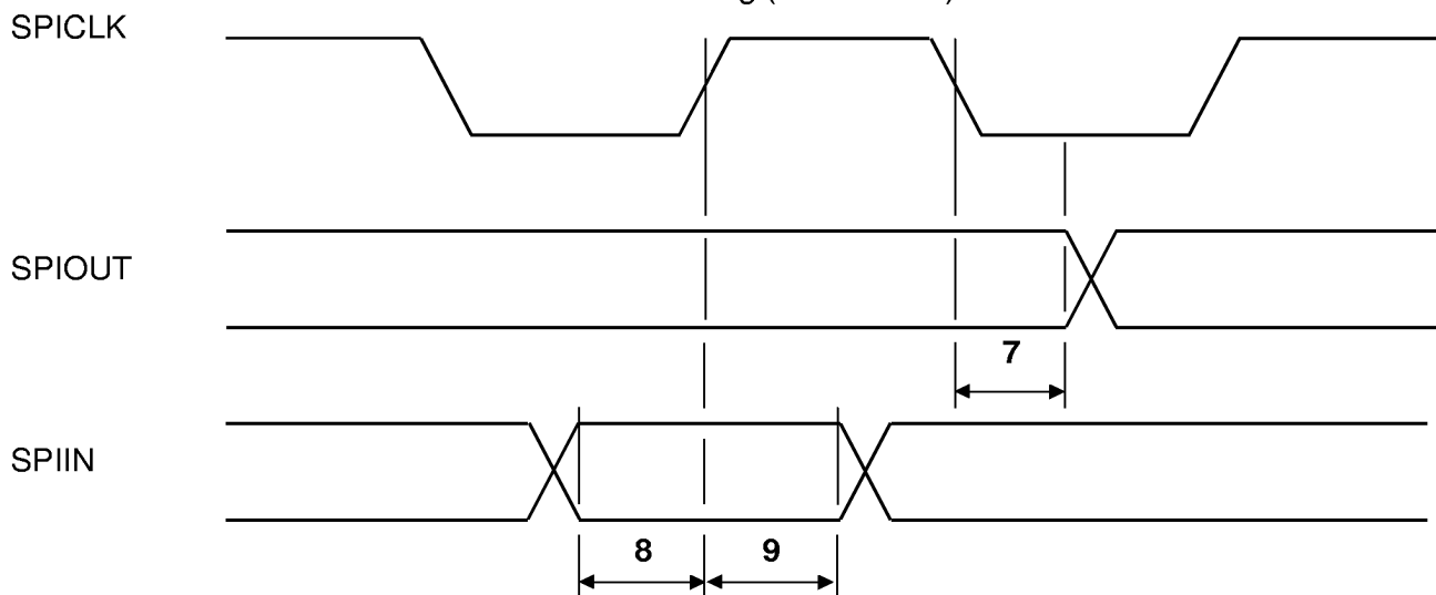
SPI Timing (PHAPOL=0)
