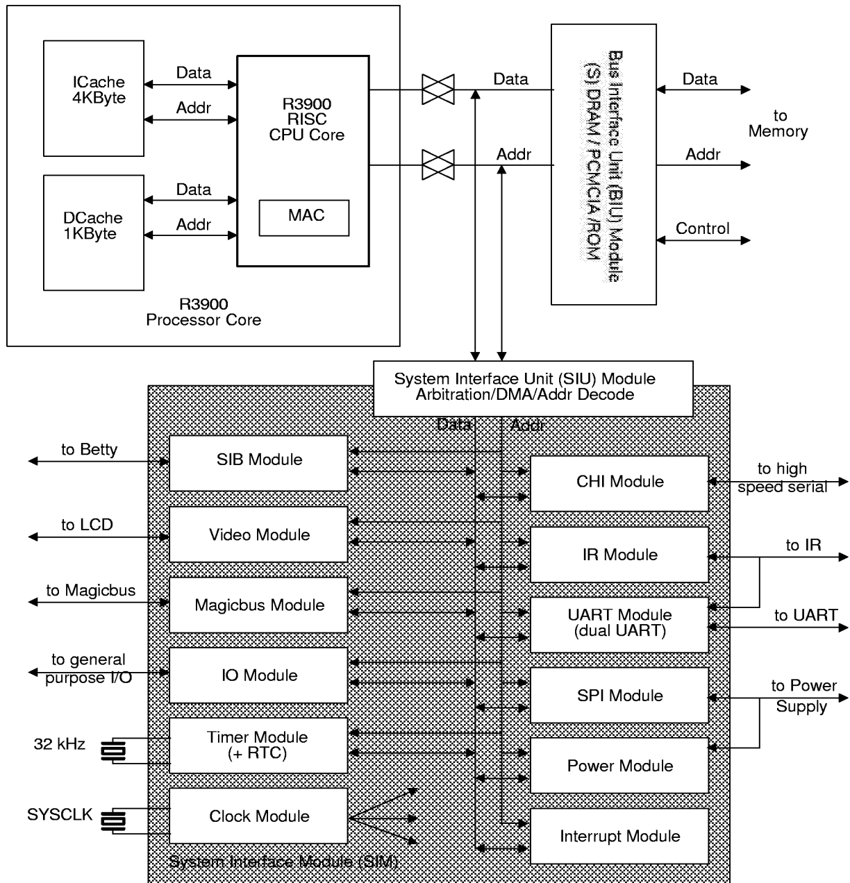
FIG. 3.2 TMPR3912U BLOCK DIAGRAM
