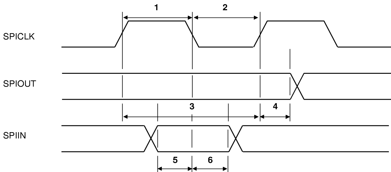
SPI Timing (PHAPOL=1)
