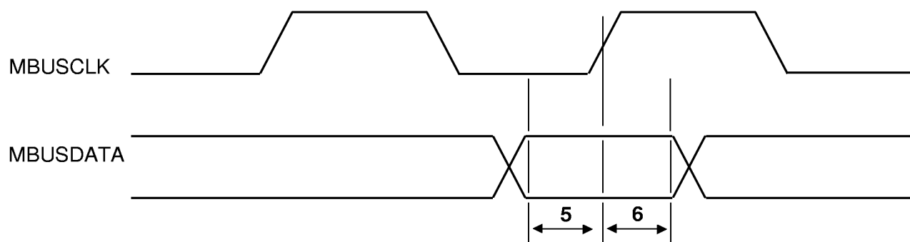
Magic Bus Input Timing (Slave, RCVPHAPOL=0)
