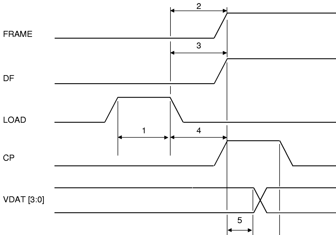
Video Timing, 4 bit non-split LCD
