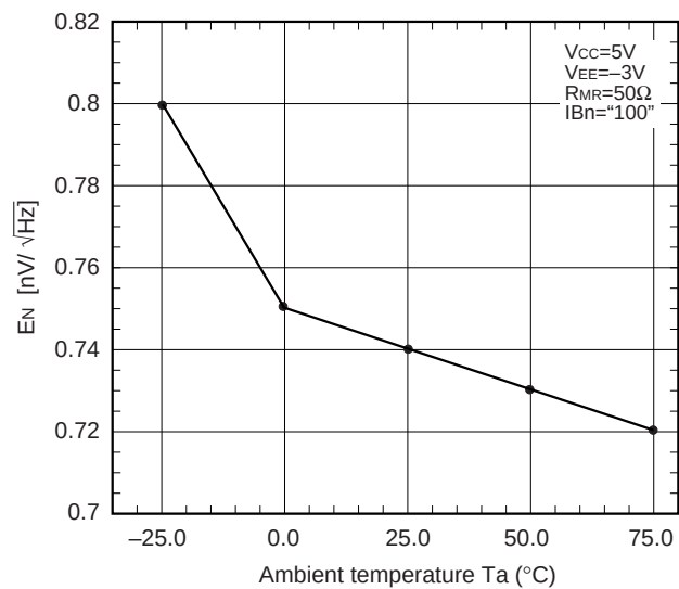
Input referred noise voltage vs Ambient temperature
