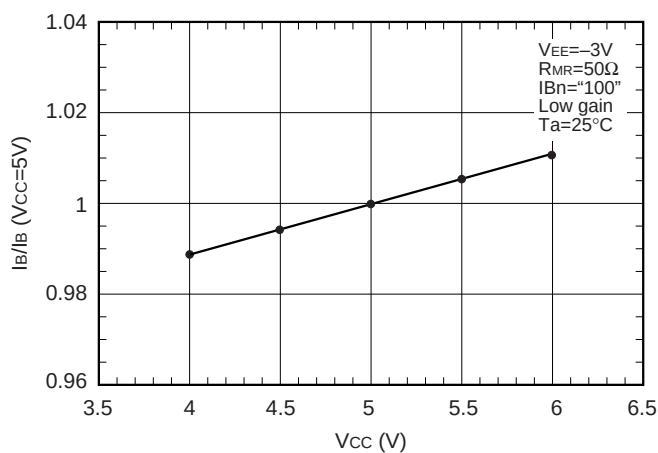
Normalized bias current vs Power supply voltage
