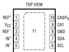
DD PACKAGE 10-LEAD (3mm × 3mm) PLASTIC DFN
