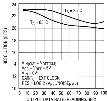
Figure 19. Resolution ( \text{Noise}_{\text{RMS}} \leq 1\text{LSB} ) vs Output Data Rate and Temperature
