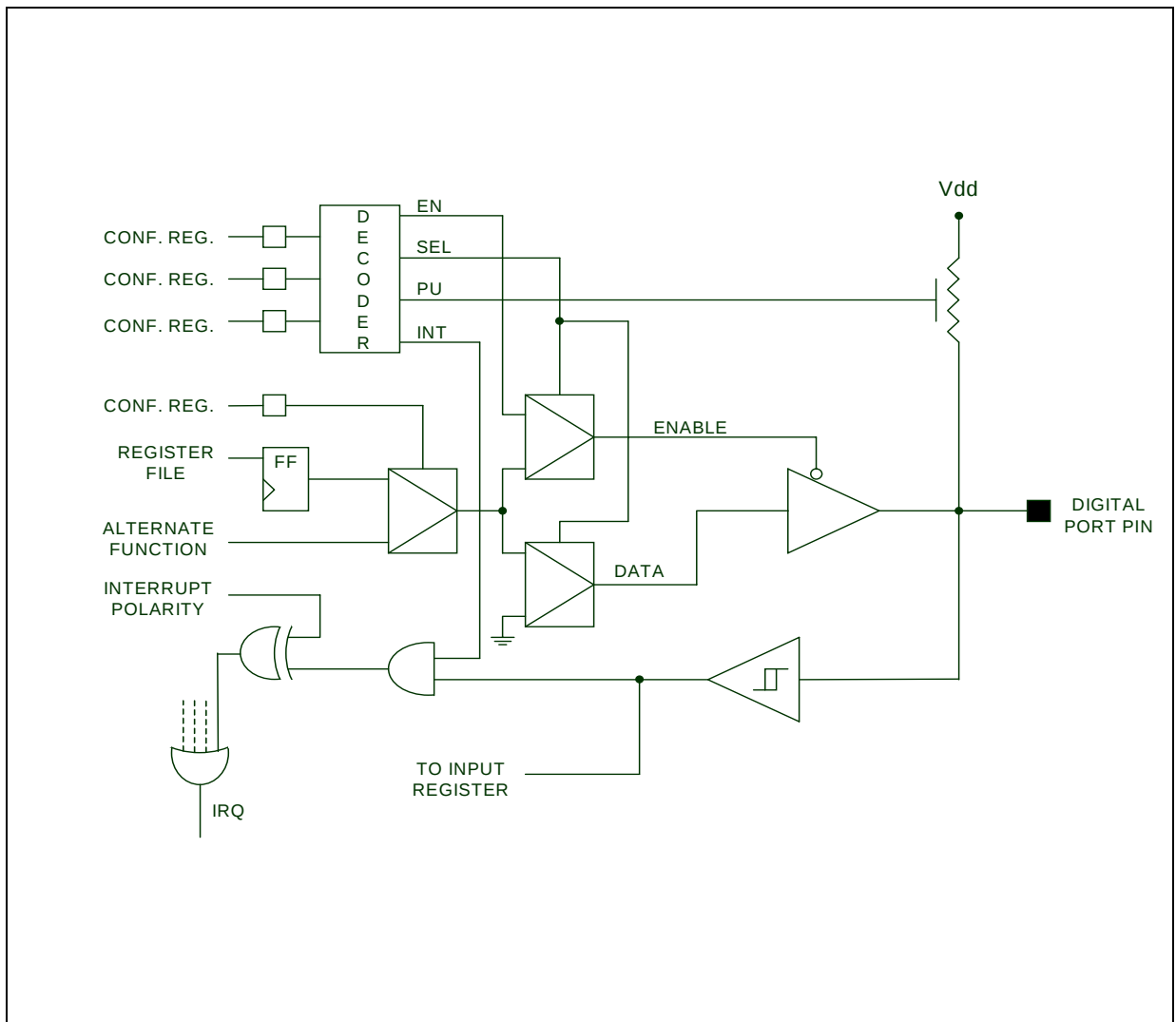
Figure 8.2 Port Pin Architecture
