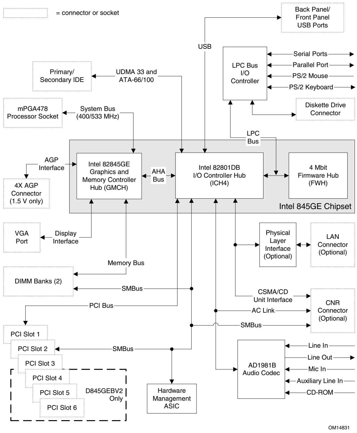
Figure 4. Block Diagram
