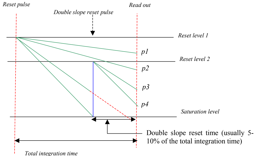
Figure 21: Dual slope diagram
