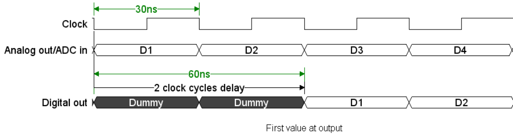
Figure 6: ADC timing
