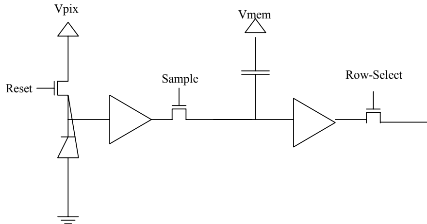
Figure 4: 6T-pixel architecture
