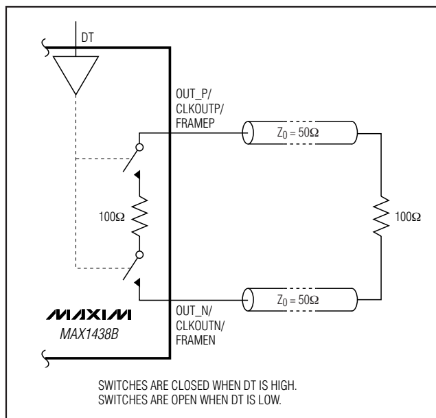
Figure 7. Double Termination
