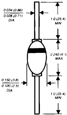
DO-204AP
