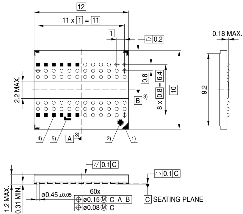
FIGURE 6 Package Outline PG-TFBGA-60
