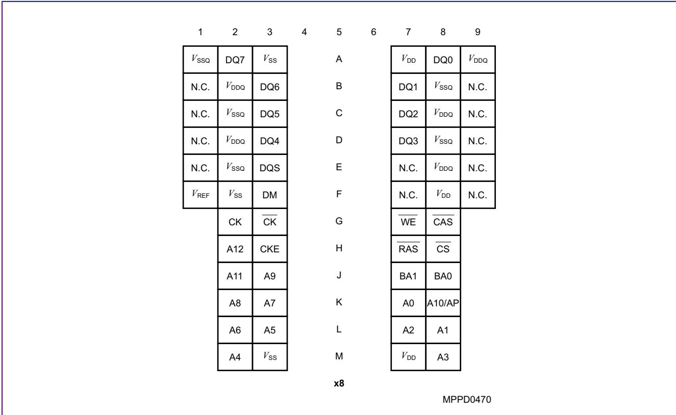
FIGURE 1 Configuration for x8 Organization, TFBGA-60, Top View
