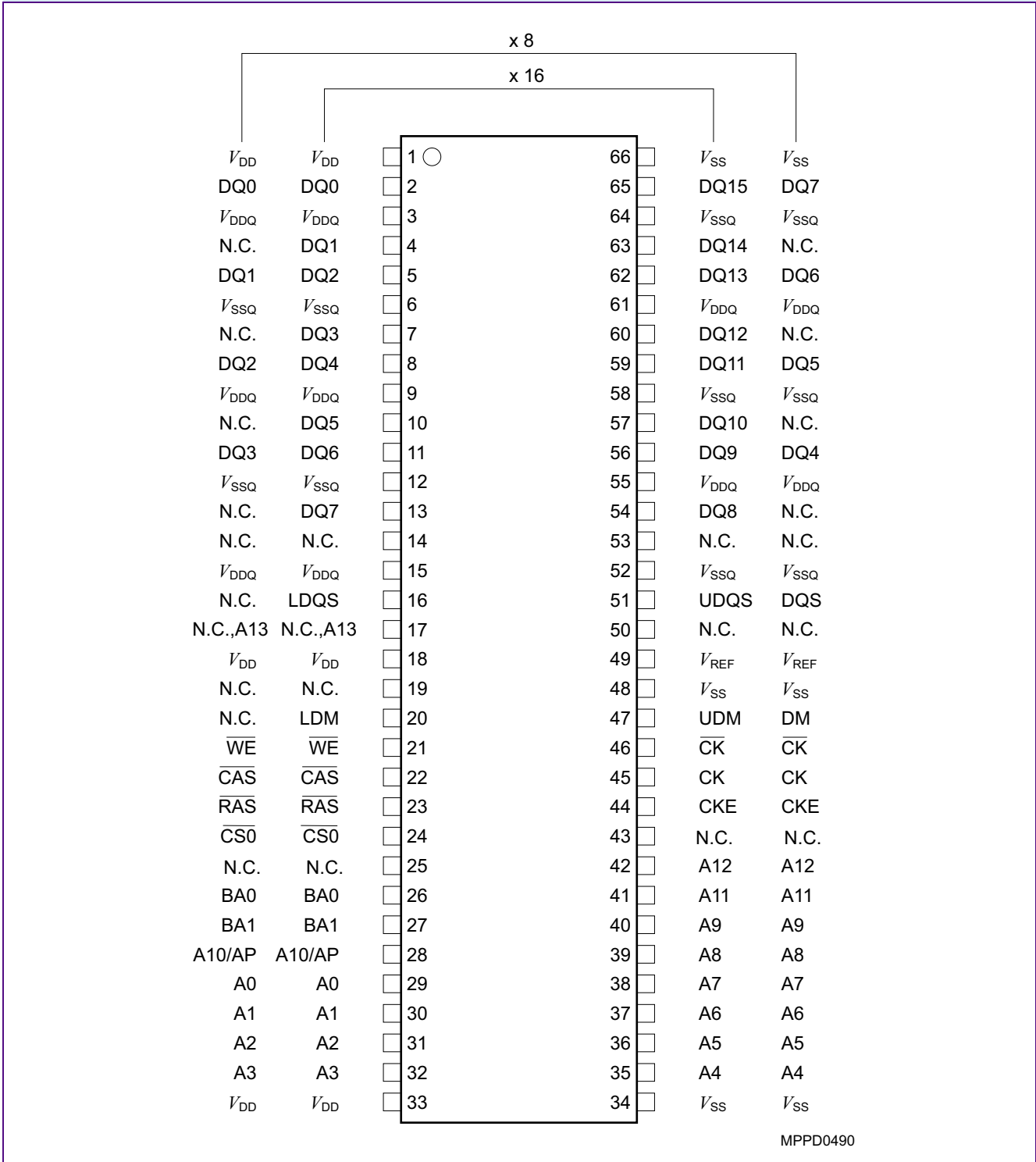
FIGURE 3 Pin Configuration TSOP1-66
