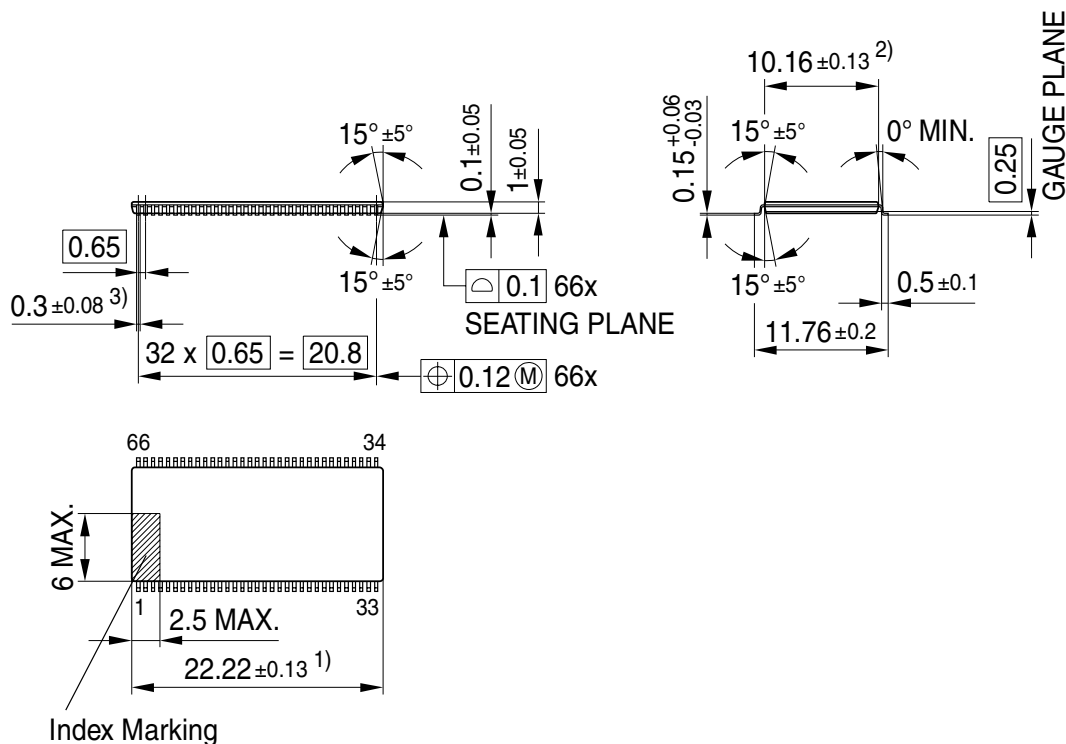
FIGURE 5 Package Outline P(G)-TSOPII-66
