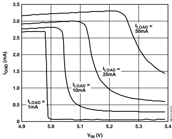
Figure 13. Ground Current vs. Input Voltage (in Dropout)
