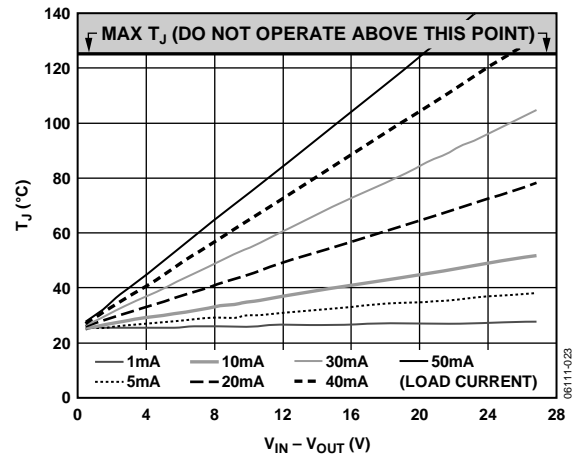
Figure 23. 100 mm 2 of PCB Copper, T_A = 25^\circ\text{C}
