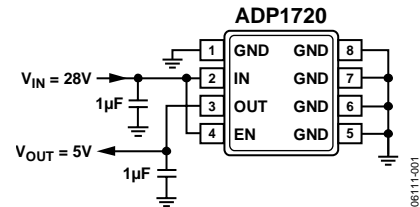
Figure 1. ADP1720 with Fixed Output Voltage, 5.0 V
