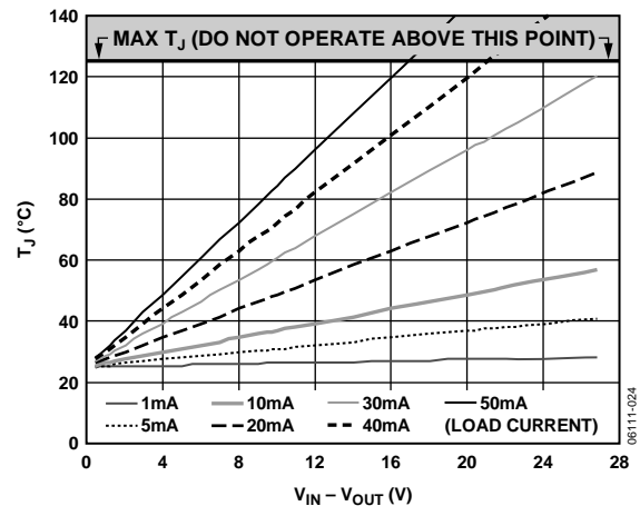
Figure 24. 0 mm 2 of PCB Copper, T_A = 25^\circ\text{C}
