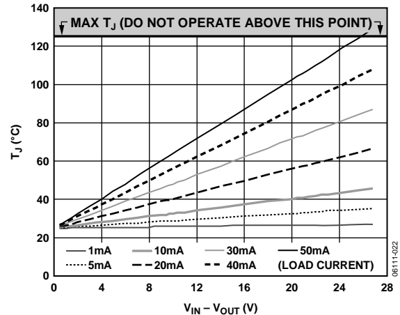
Figure 22. 300 mm 2 of PCB Copper, T_A = 25^\circ\text{C}
