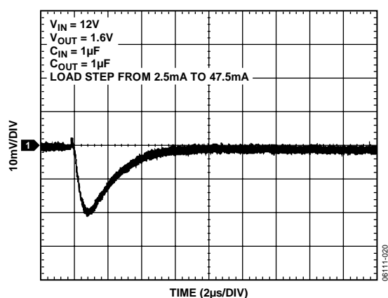
Figure 20. Output Transient Response
