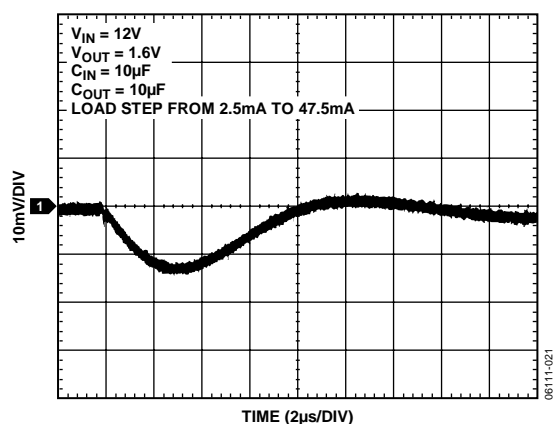
Figure 21. Output Transient Response
