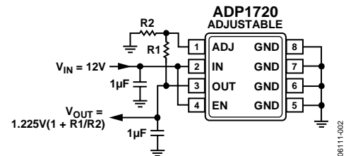
Figure 2. ADP1720 with Adjustable Output Voltage, 1.225 V to 5.0 V
