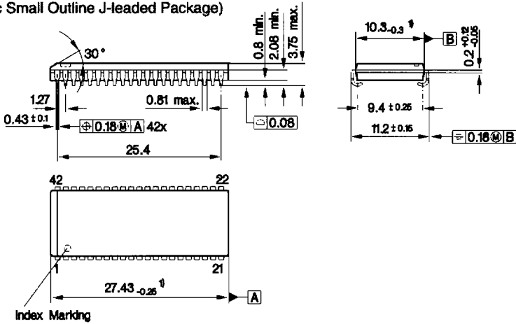
P-SOJ-42 (400 mil) (Plastic Small Outline J-led Package)
