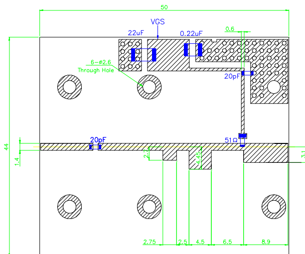
Test Fixture
